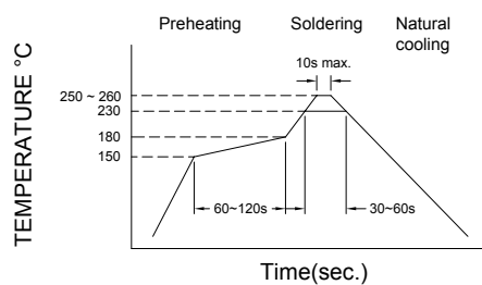
Figure 1. Re-flow Soldering
