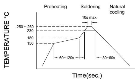
Figure 1. Re-flow Soldering
