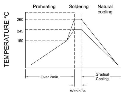
Figure 2. Wave Soldering
