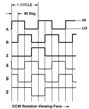
Figure 1 Output Waveform
