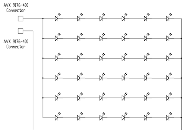
Figure 11. Electrical circuit diagram for L235-xyyyAHLCCBBAC0.
