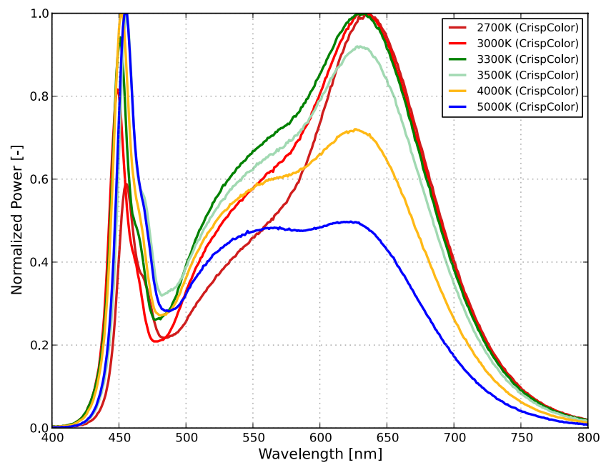
Figure 1. Typical normalized power vs. wavelength for 90CRI LUXEON 3535L with CrispColor Technology at 100mA, T_j=25^{\circ}\text{C} .
