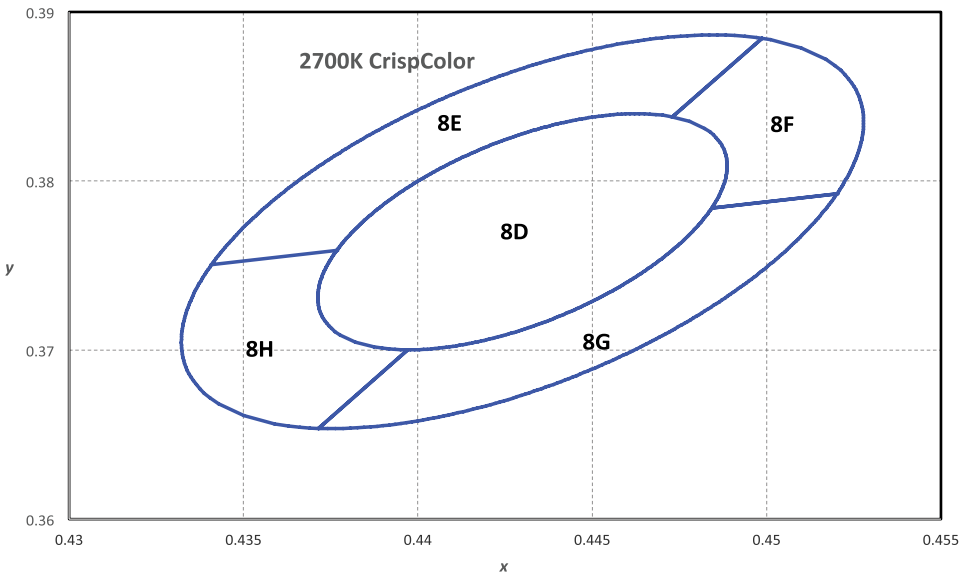
Figure 8a. 1/5 th color bin structure for LUXEON 3535L with CrispColor Technology 2700K at T j =25°C.
