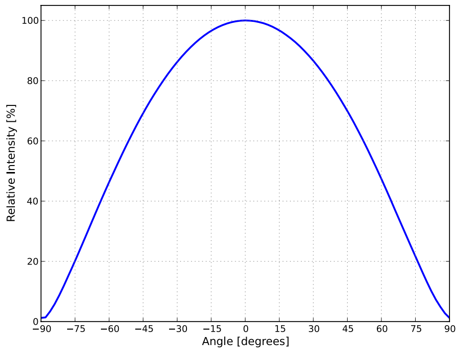
Figure 4. Typical radiation pattern for L130-xxxx001400001 at 60mA, T j =25°C.
