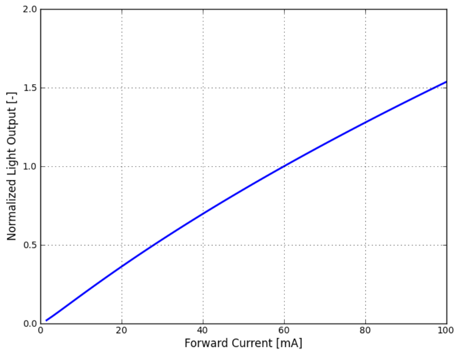
Figure 2b. Typical normalized light output vs. forward current for L130-xxxx001400001 at T_j=25^{\circ}\text{C} .
