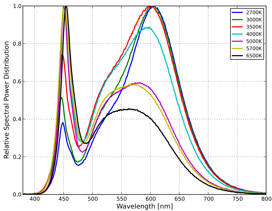
Figure 1b. Typical normalized power vs. wavelength for L130-xx80001400001 at 60mA, T j =25°C.
