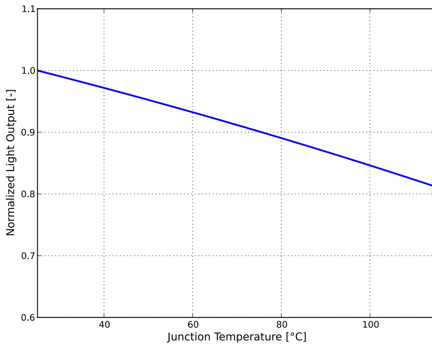
Figure 2a. Typical normalized light output vs. junction temperature for L130-xxxx001400001 at 60mA.
