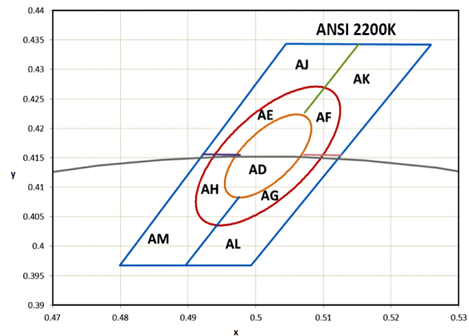
Figure 7a. Color bin structure for LUXEON 3014 2200K, hot-color targeted at T_j=65^{\circ}\text{C} .
