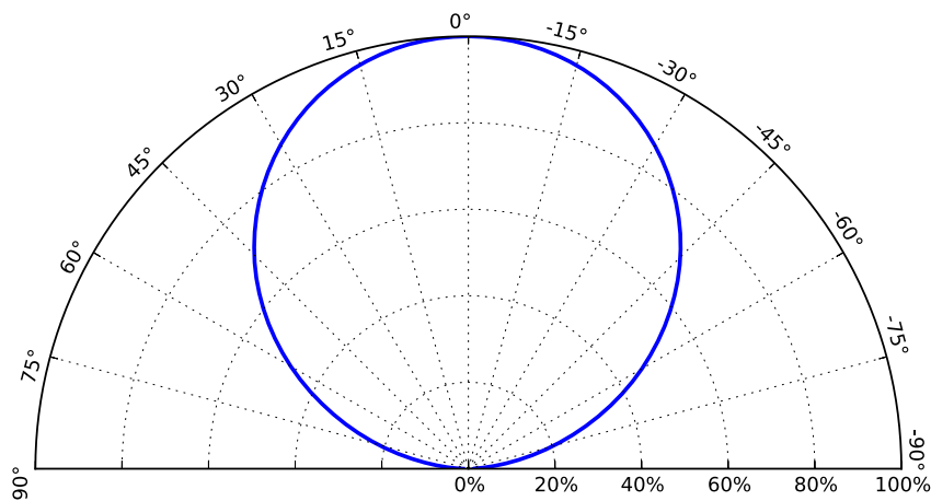
Figure 5. Typical polar radiation pattern for L130-xxxx001400001 at 60mA, T j =25°C.
