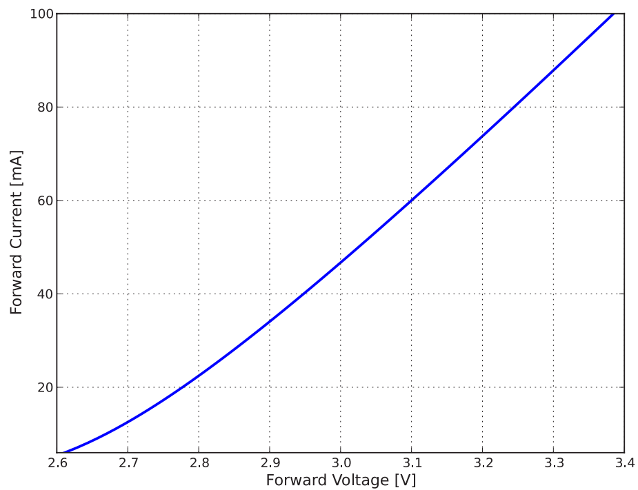
Figure 3. Typical forward current vs. forward voltage for L130-xxxx001400001 at T_j=25^{\circ}\text{C} .
