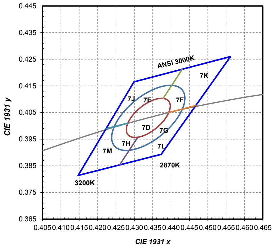
Figure 15. 3000K 1/9 th color bin structure.
