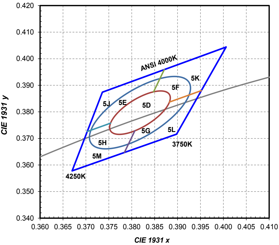
Figure 17. 4000K 1/9 th color bin structure.
