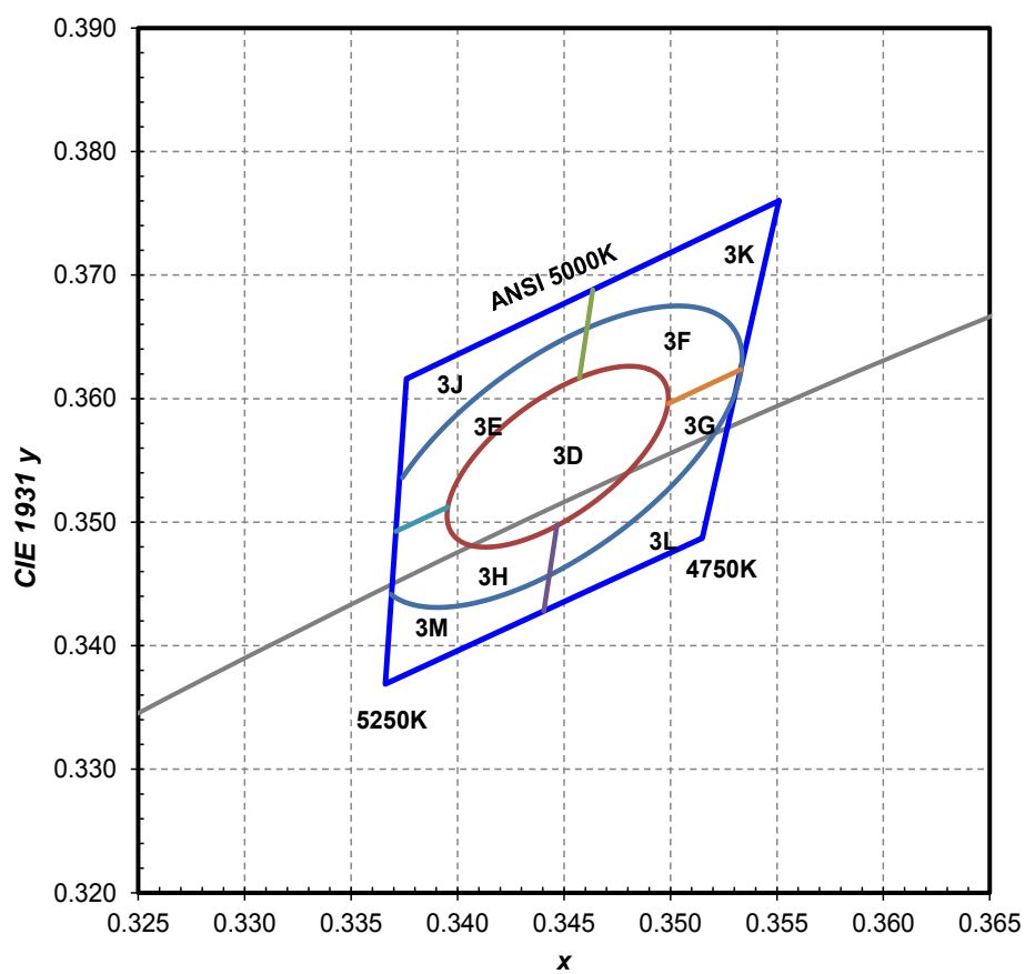
Figure 18. 5000K 1/9 th color bin structure.
