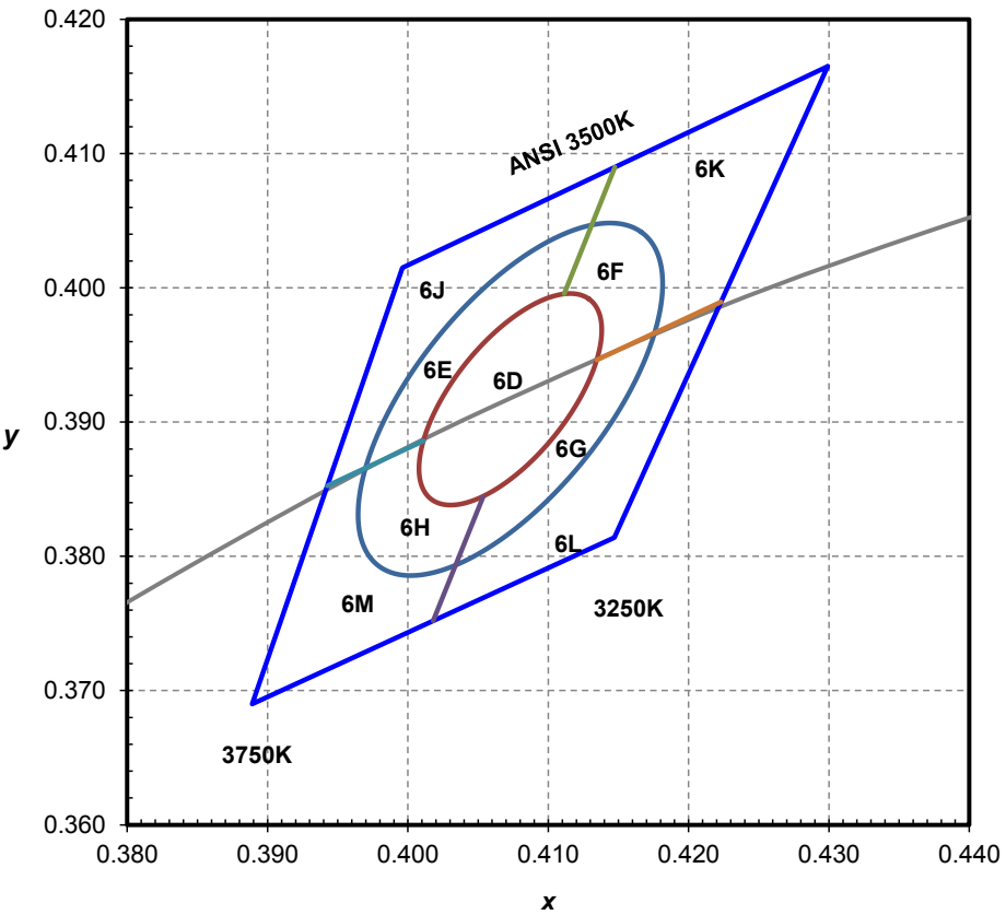
Figure 16. 3500K 1/9 th color bin structure.
