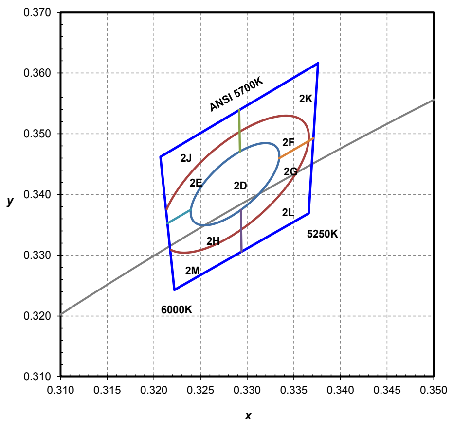
Figure 19. 5700K 1/9 th color bin structure.
