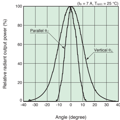
Figure 3: Directivity (typ.)
