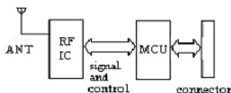
KYL-300L Principle map
