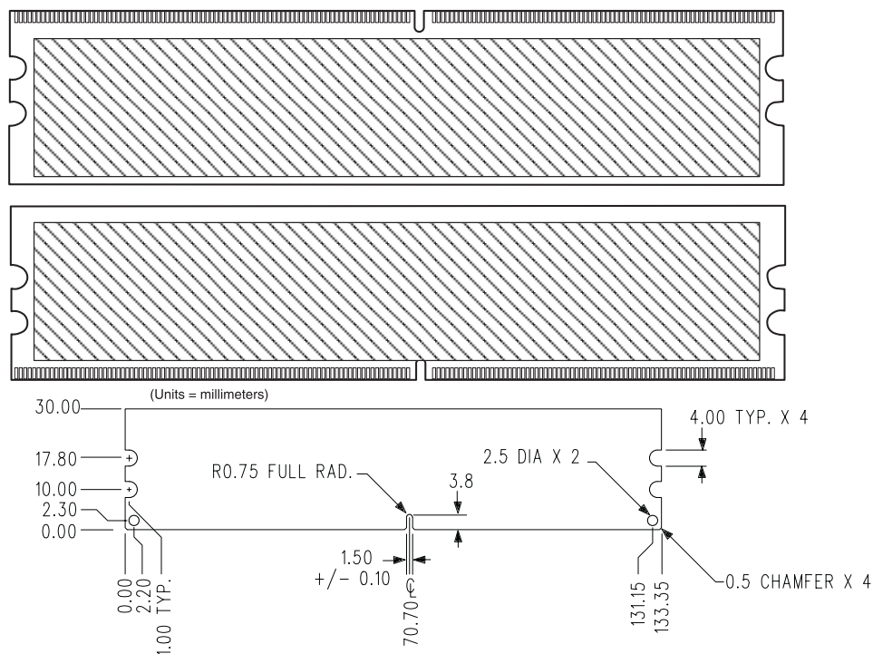
Figure 1: KVR400D2S4R3K2/4G 240-Pin DIMM
