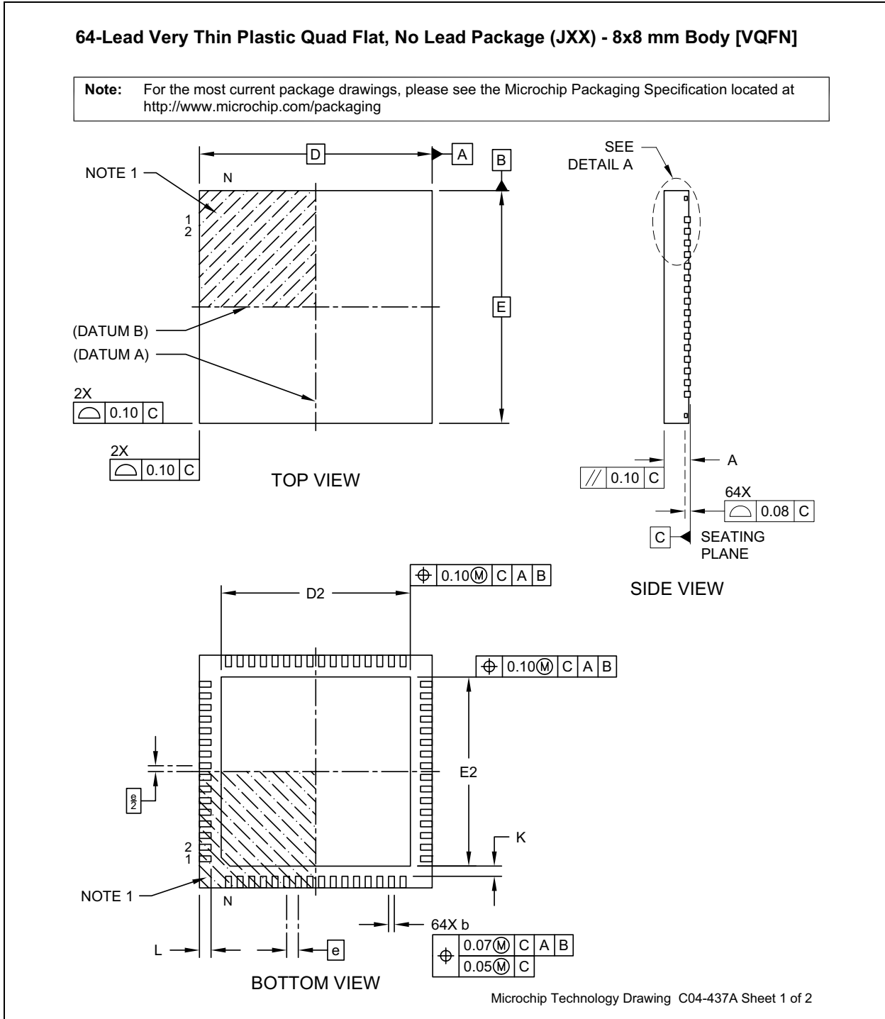
FIGURE 8-1: PACKAGE (DRAWING)
