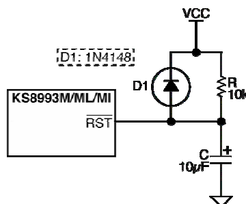
Figure 25. Recommended Circuit for Interfacing with CPU/FPGA Reset
