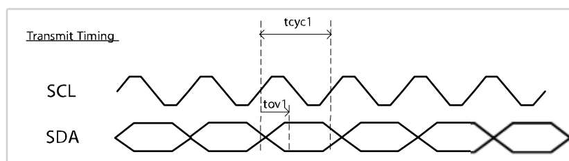
Figure 14. EEPROM Interface Output Timing Diagram
