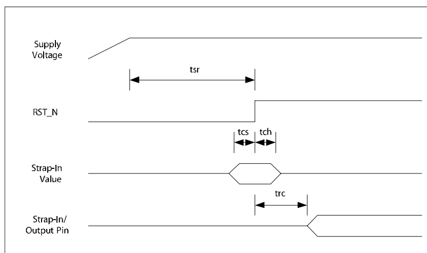
Figure 23. Reset Timing
