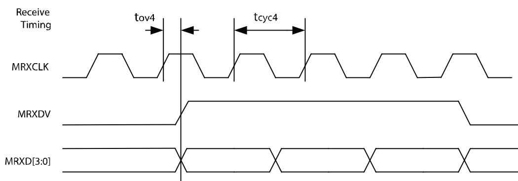
Figure 20. PHY-Mode MII Timing – Data Input to MII
