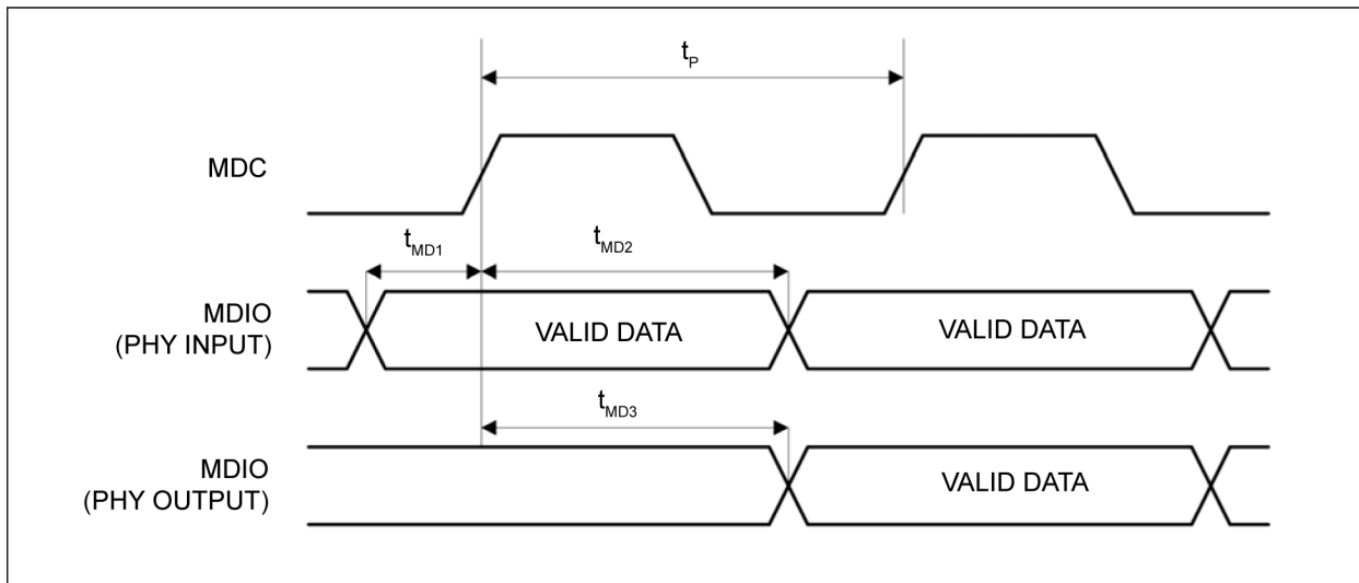
FIGURE 7-14: MDC/MDIO TIMING
