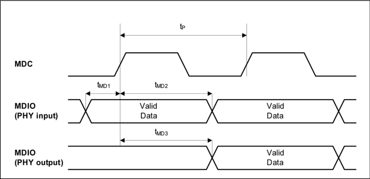
FIGURE 7-14: MDC/MDIO TIMING
