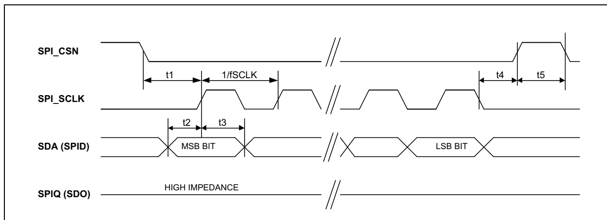
FIGURE 7-11: SPI INPUT TIMING
