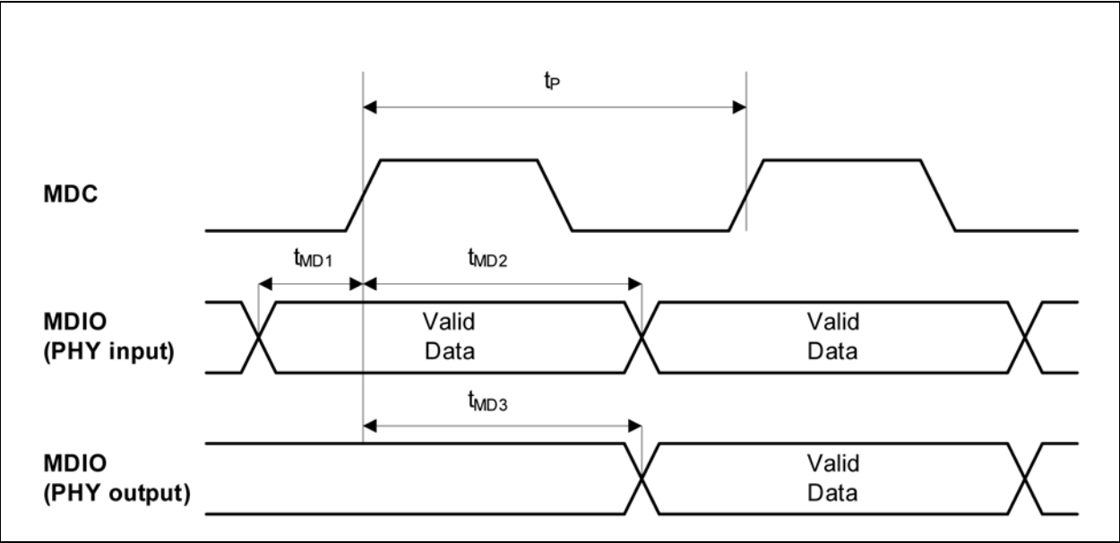
FIGURE 7-16: MDC/MDIO TIMING
