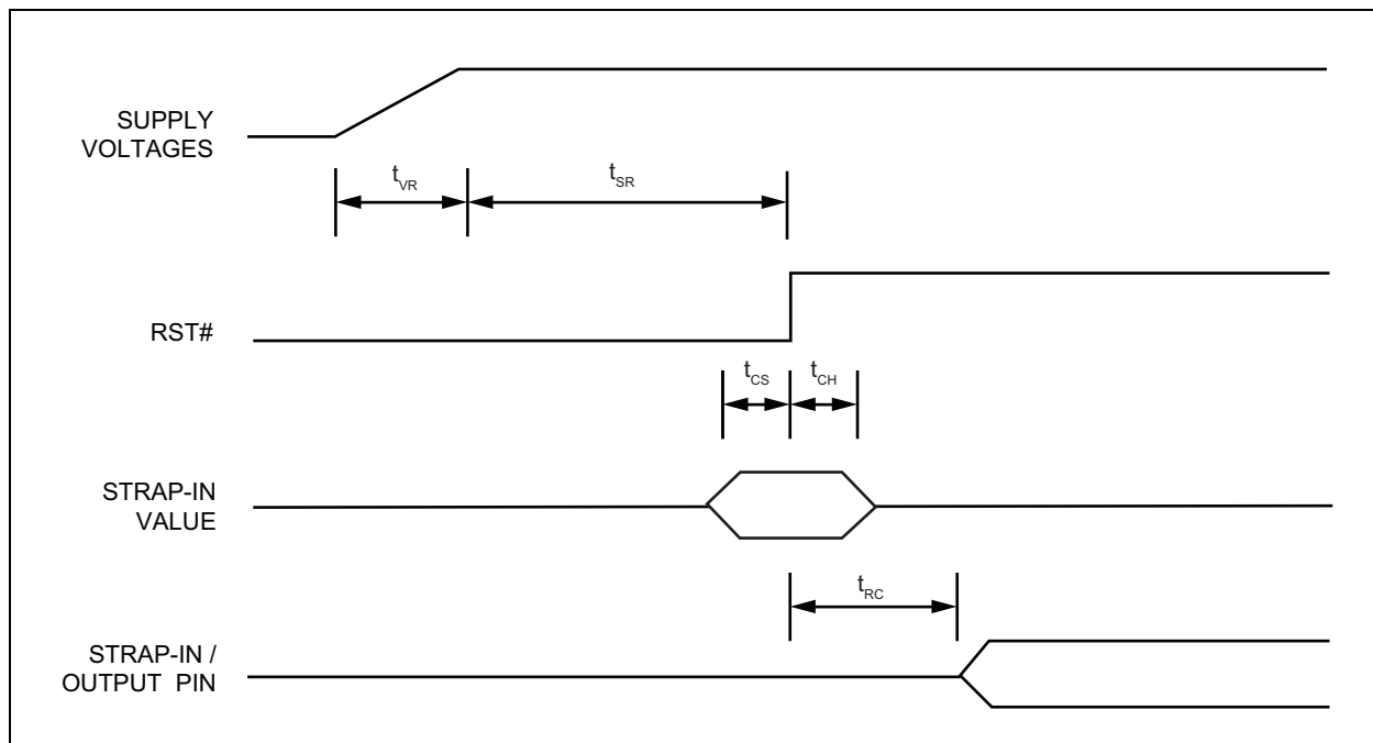
FIGURE 7-17: RESET TIMING
