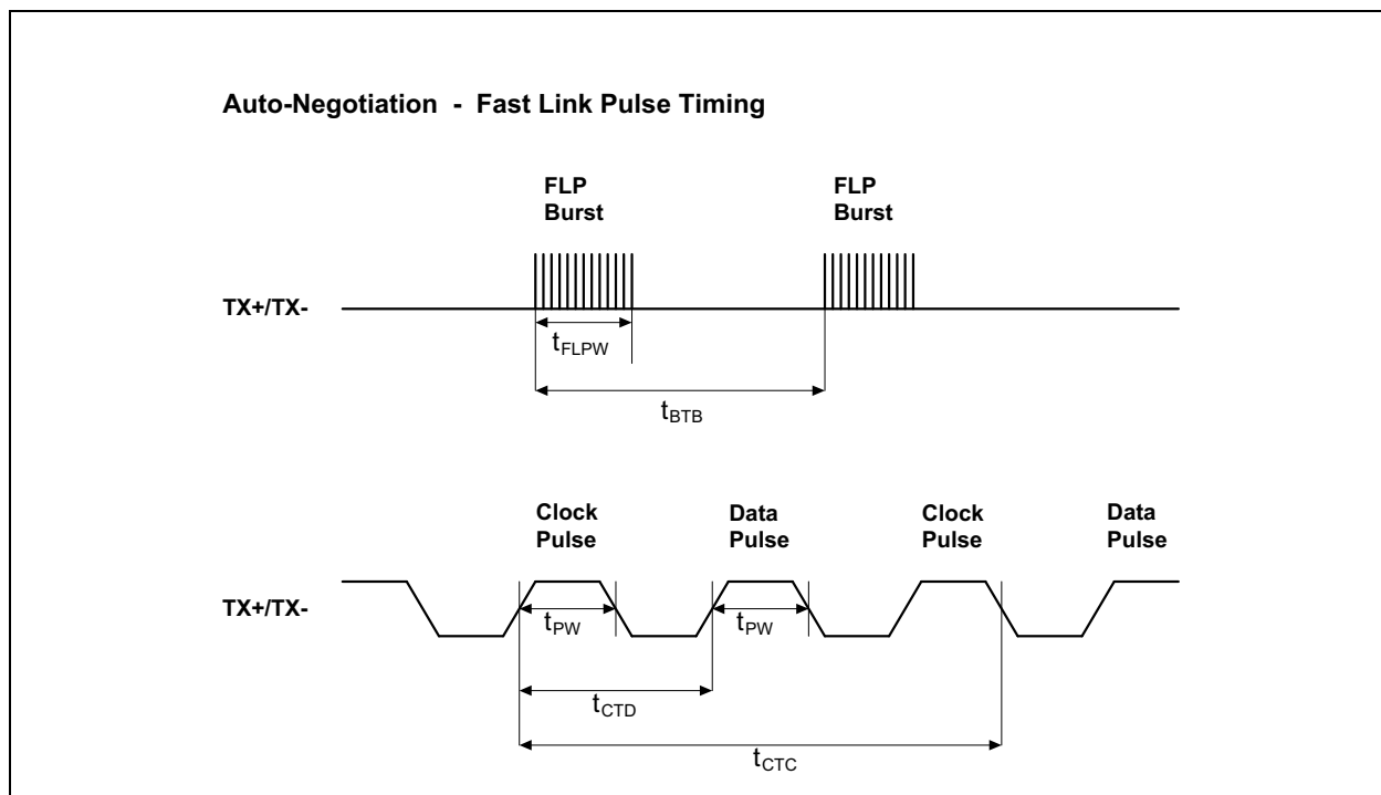
FIGURE 7-15: AUTO-NEGOTIATION TIMING
