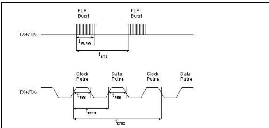
Figure 23. Auto-Negotiation Timing
