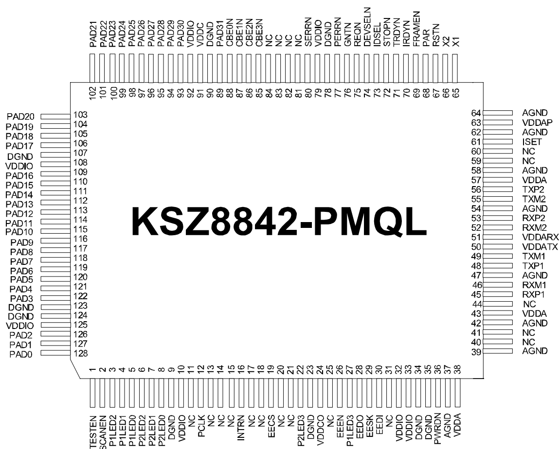
Figure 2. KSZ8842-PMQL 128-Pin PQFP (Top View)
