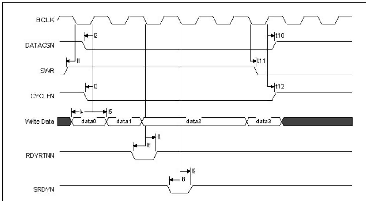
Figure 17. Synchronous Burst Write Cycles – VLBSN = 1
