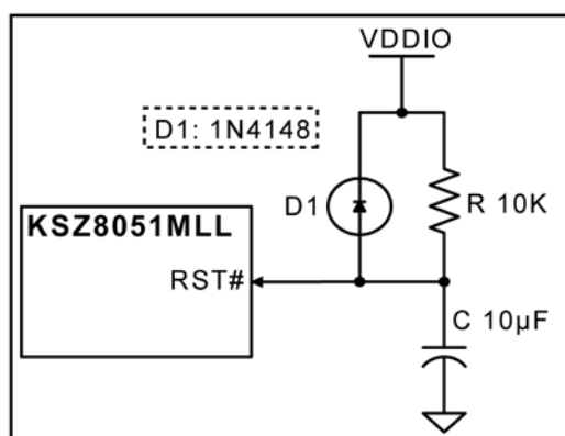
Figure 15. Recommended Reset Circuit
