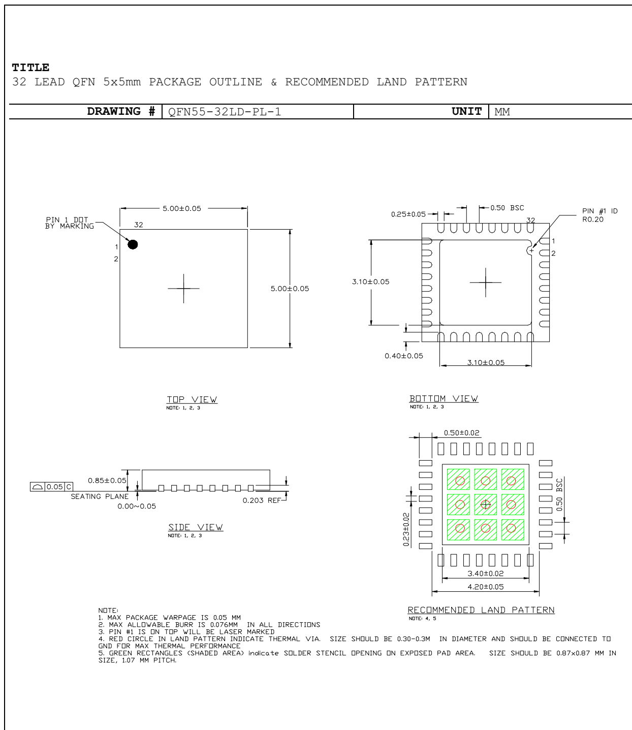
FIGURE 10-1: 32-LEAD QFN 5X5 PACKAGE
