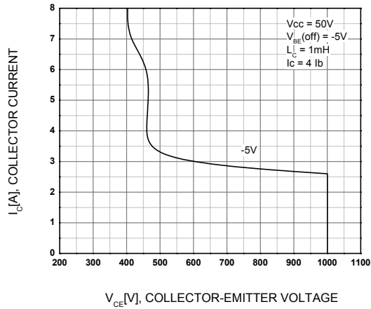
Figure 15. Reverse Bias Safe Operating
