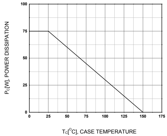
Figure 16. Power Derating
