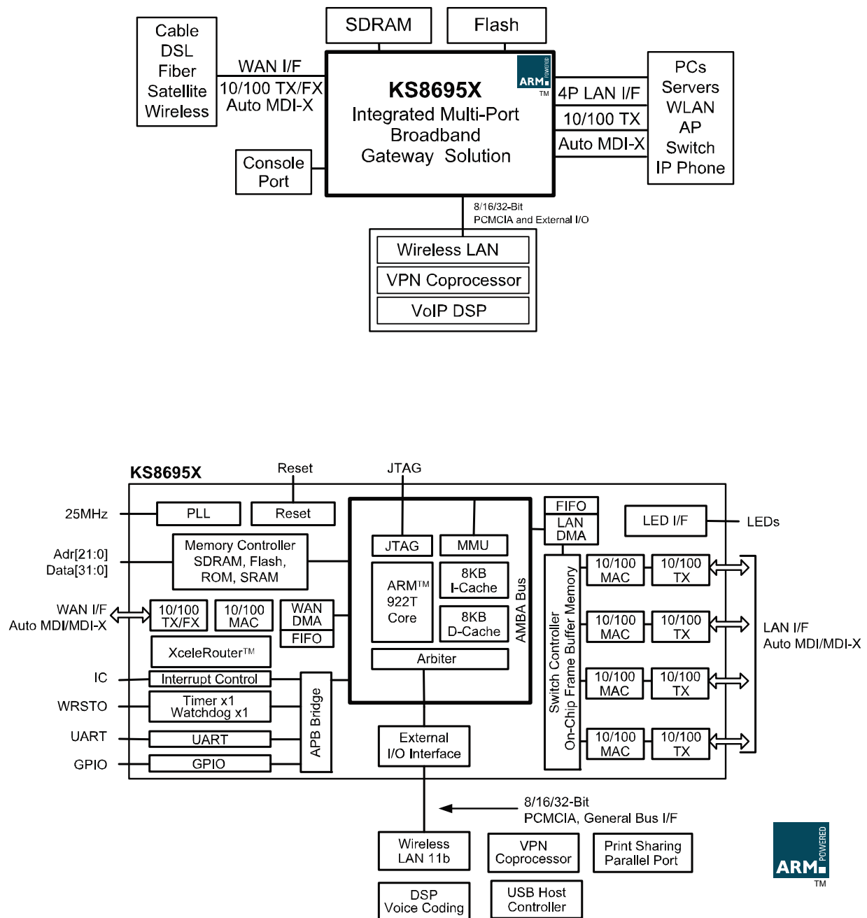
Figure 1. KS8695X Applications
