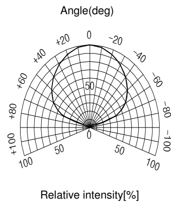
Radiant Pattern
