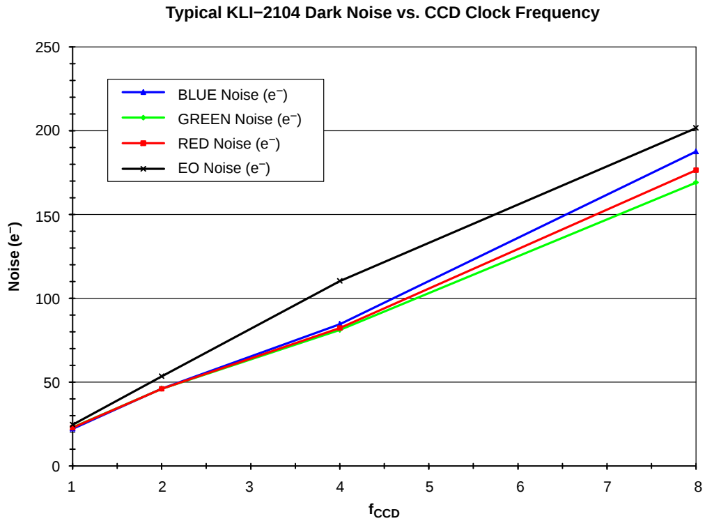
Figure 19. Typical KLI-2104 Dark Noise vs. CCD Clock Frequency
