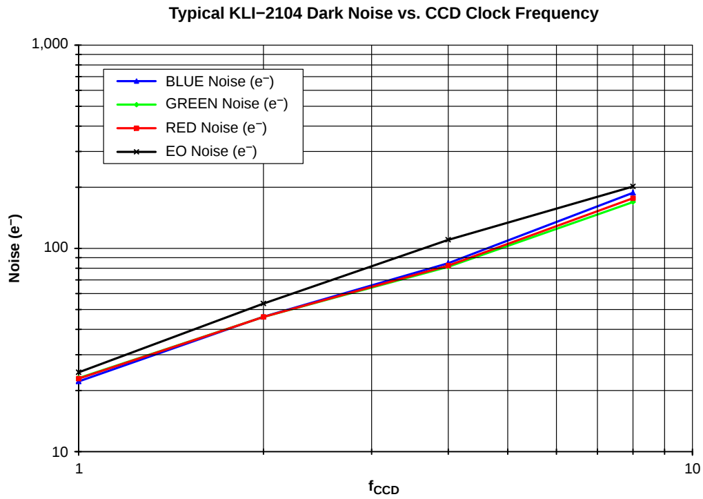
Figure 18. Typical KLI-2104 Dark Noise vs. CCD Clock Frequency
