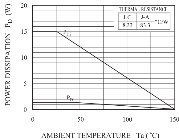
Fig.11 P_D - T_a (PI-Type : TO-220IS-4)
