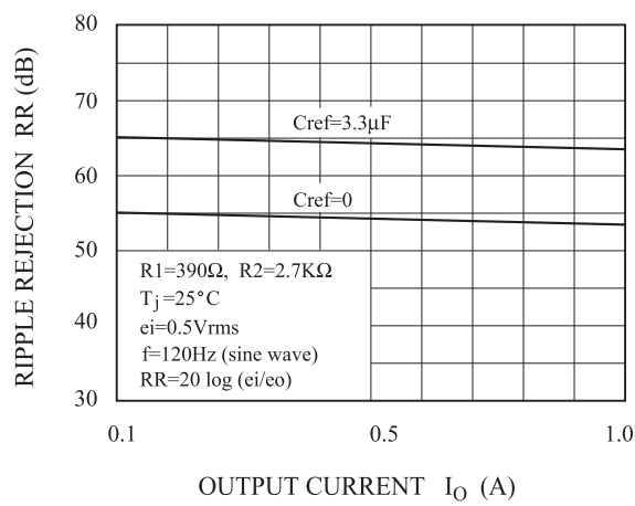
Fig. 9 I_O - RR
