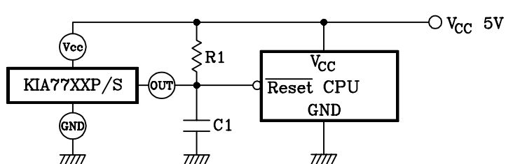
(2) CPU RESETTING
