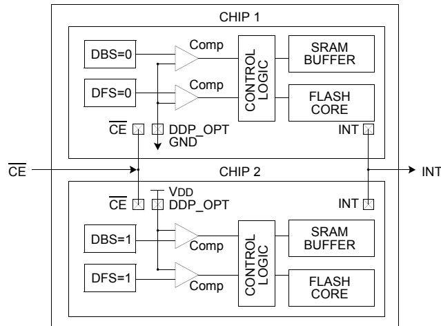
Figure 4. Chip selection method in DDP
