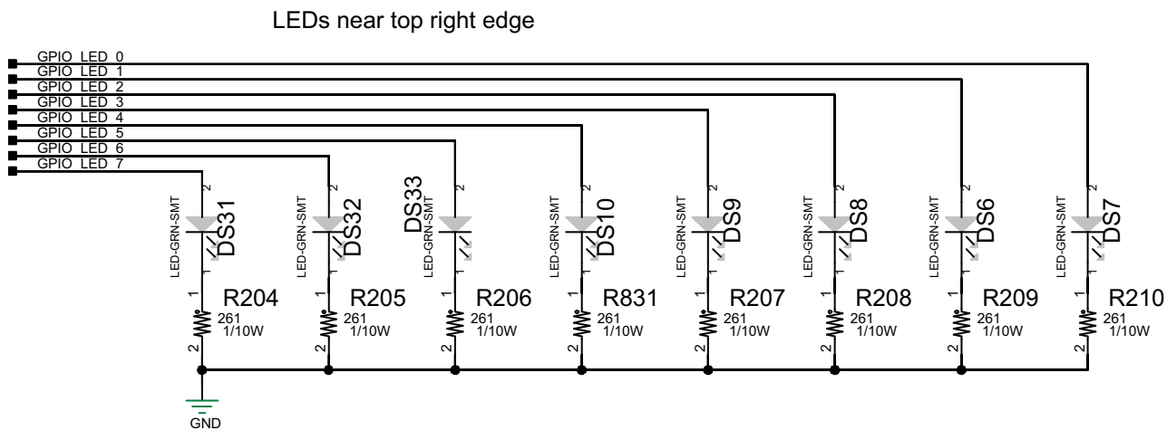
Figure 1-24: User LEDs
