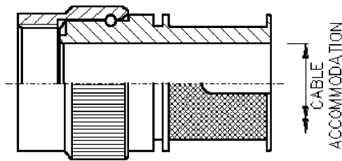
STRAIGHT BACKSHELL
