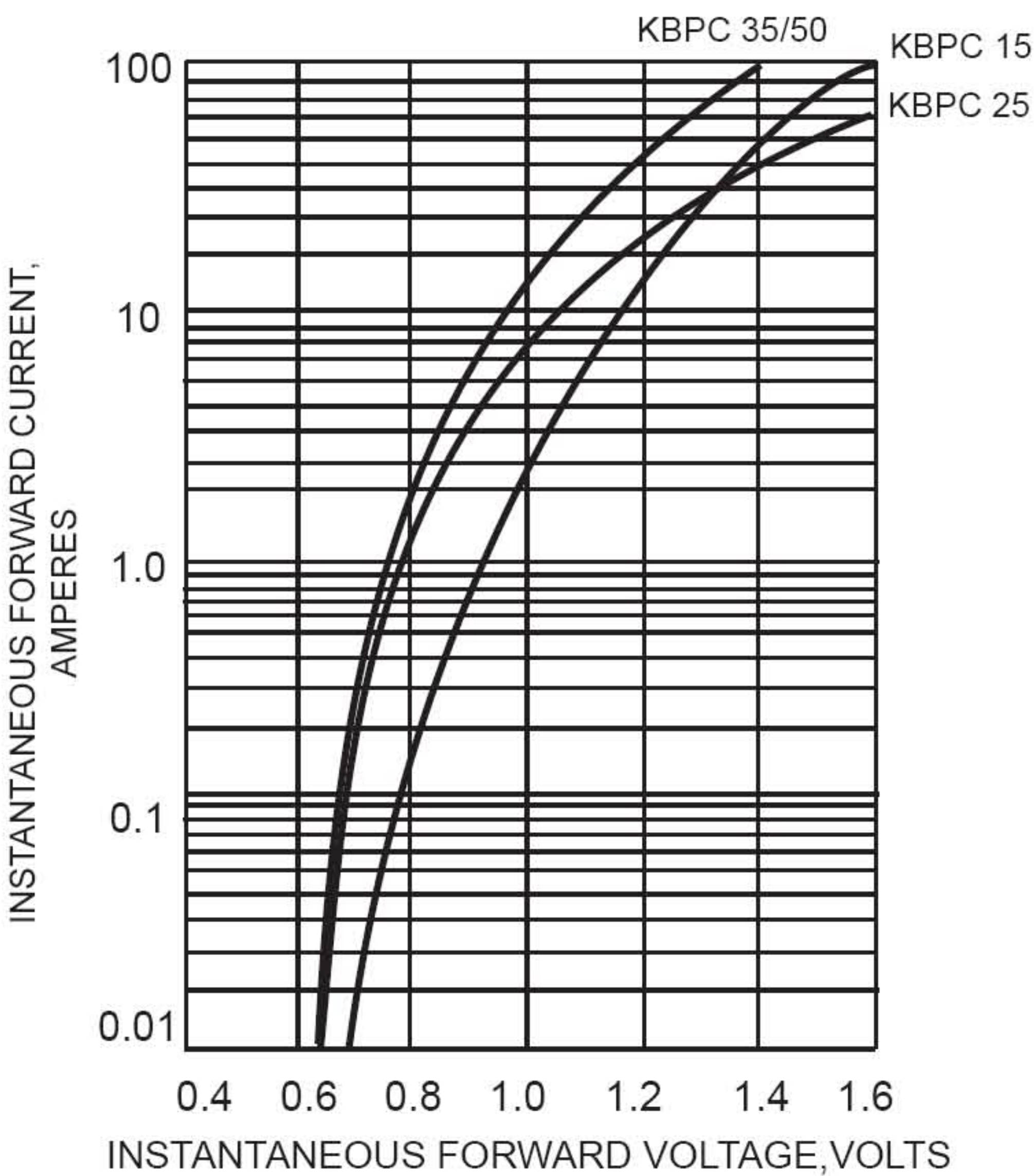
FIG.3-TYPICAL FORWARD CHARACTERISTICS
