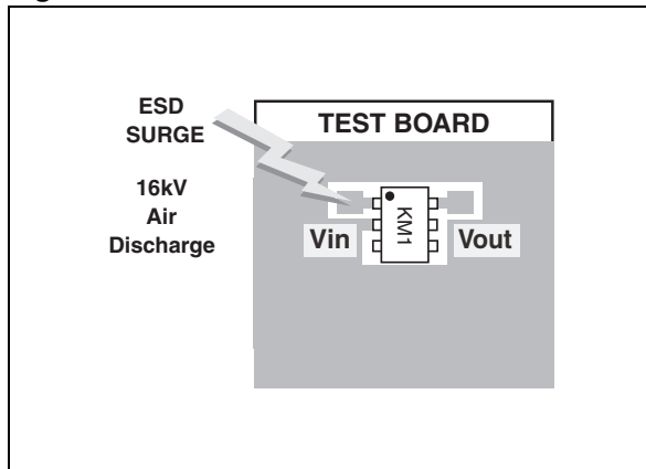
Figure 5: Measurement conditions
