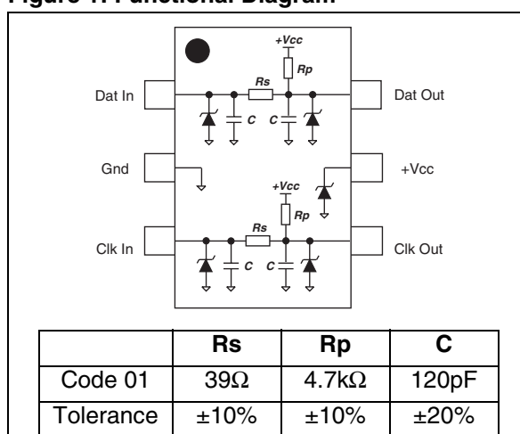
Figure 1: Functional Diagram
