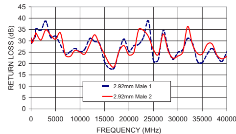
KBL-2FT-LOW+ RETURN LOSS
