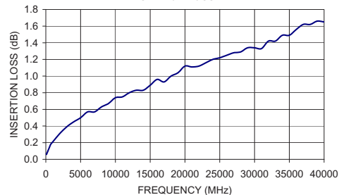
KBL-2FT-LOW+ INSERTION LOSS
