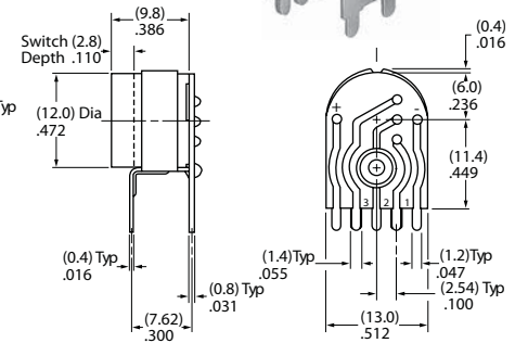
AT077 Single Pole Right Angle PC Terminals
