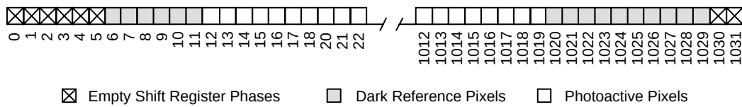
Figure 14. Frame Timing – Single Register Readout
