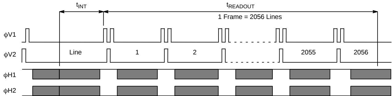
Figure 7. Frame Timing
