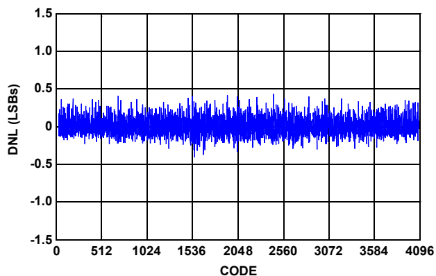
FIGURE 11. DIFFERENTIAL NONLINEARITY
