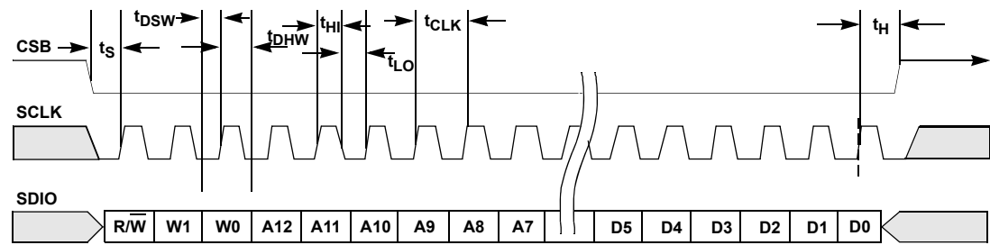
SPI WRITE
