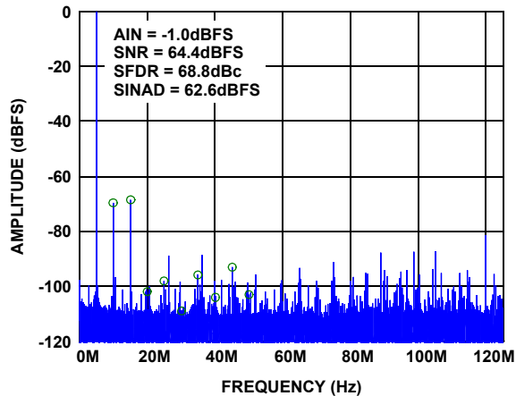
FIGURE 18. SINGLE-TONE SPECTRUM AT 495MHz
