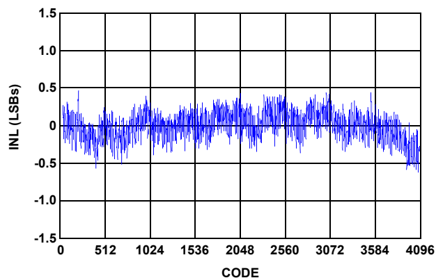
FIGURE 12. INTEGRAL NONLINEARITY
