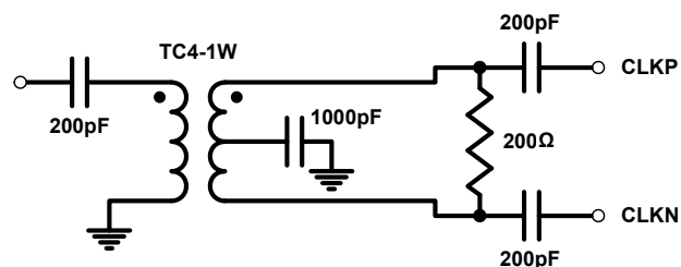
FIGURE 30. RECOMMENDED CLOCK DRIVE
