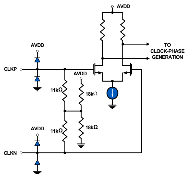
FIGURE 43. CLOCK INPUTS
