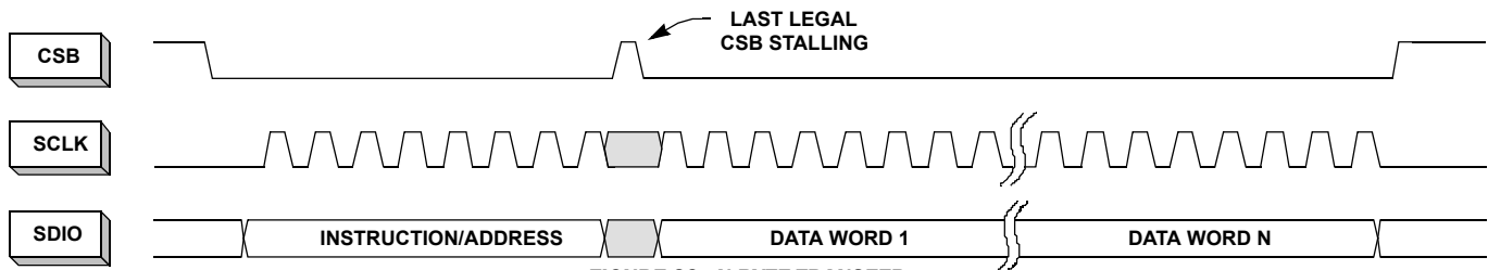
FIGURE 39. N-BYTE TRANSFER
