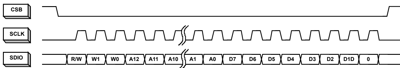
FIGURE 34. MSB-FIRST ADDRESSING
