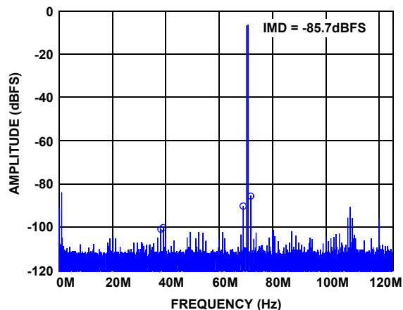
FIGURE 20. TWO-TONE SPECTRUM AT 70MHz
