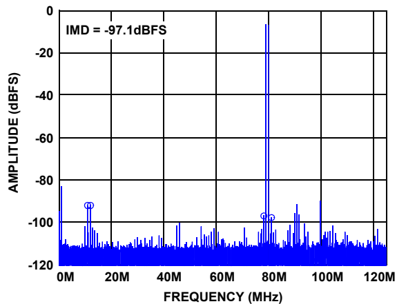
FIGURE 21. TWO-TONE SPECTRUM AT 170MHz
