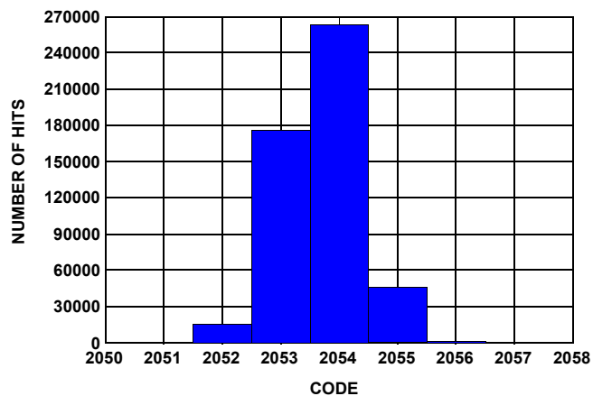
FIGURE 14. NOISE HISTOGRAM
