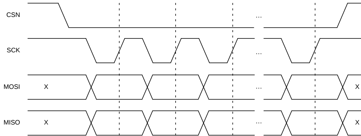
Figure 25. CPOL = 1 and CPHA = 1 Configuration
