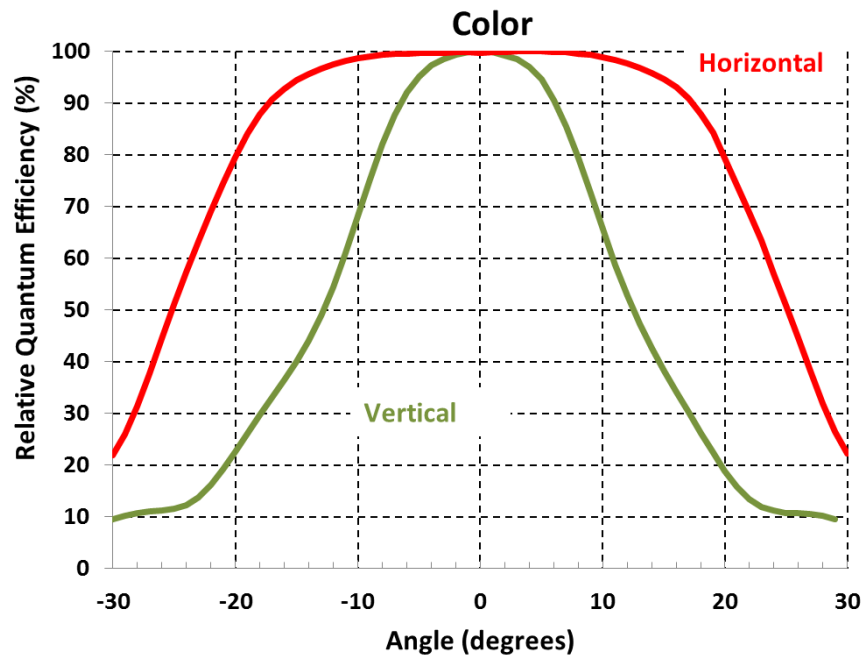
Figure 7. Bayer Relative Angular QE (with Microlens)
