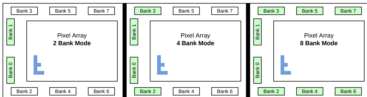
Figure 22. LVDS Bank Labeling
