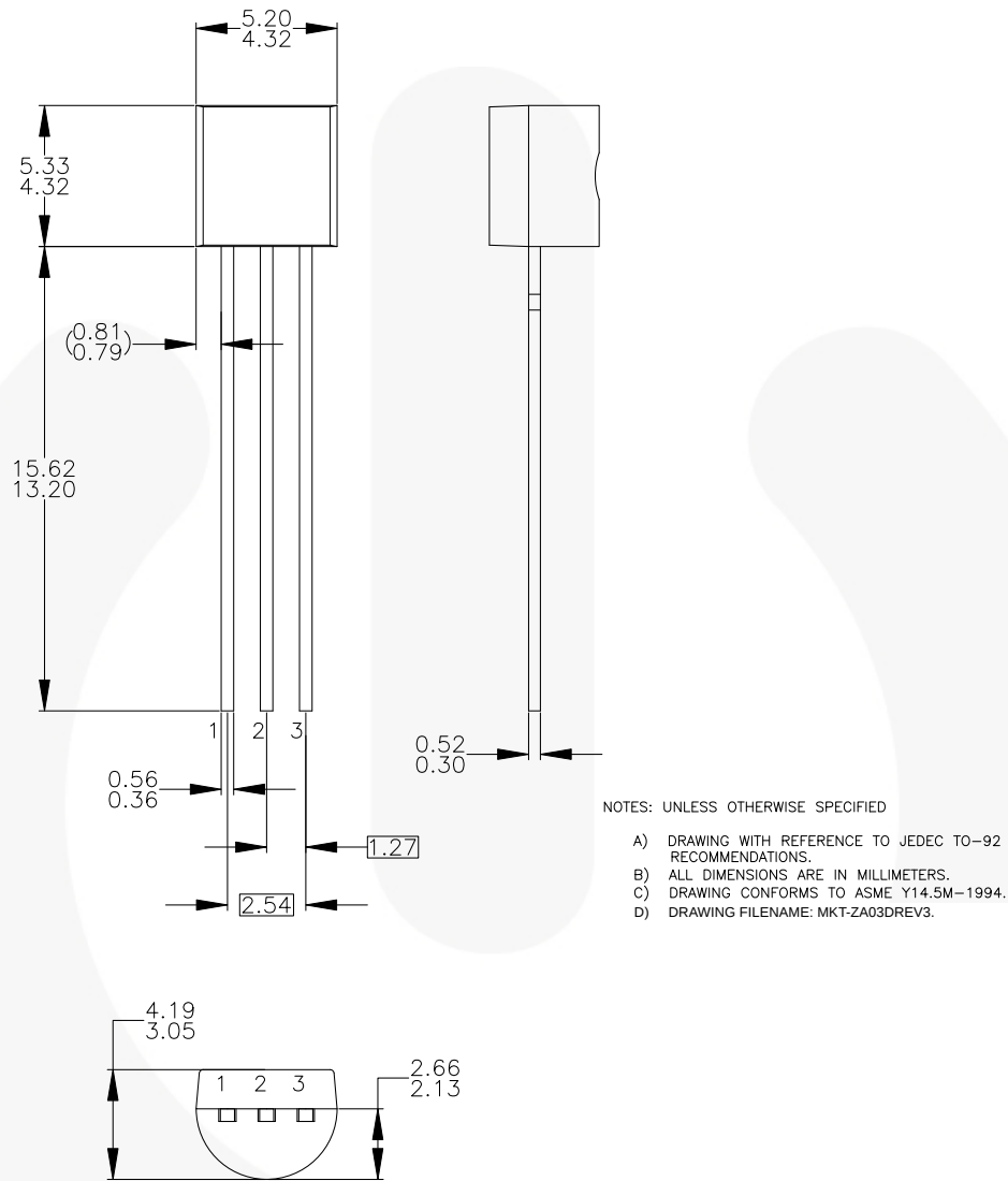
Figure 17. 3-Lead, TO-92, Molded, Standard Straight Lead
