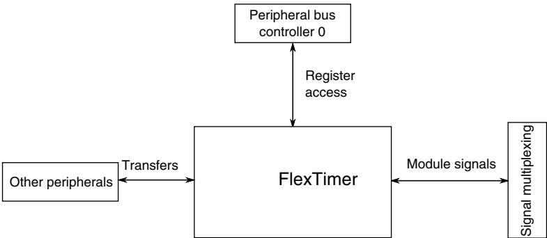
Figure 3-44. FlexTimer configuration
