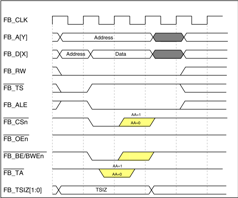
Figure 29-37. Basic Write-Bus Cycle (No Wait States)
