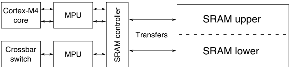
Figure 3-23. SRAM configuration
