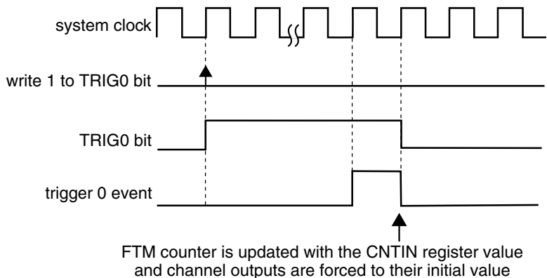
Figure 39-224. FTM Counter Synchronization with (SYNCMODE = 0), (HWTRIGMODE = 0), (REINIT = 1), (PWMSYNC = 1), and (a Hardware Trigger Was Used)
