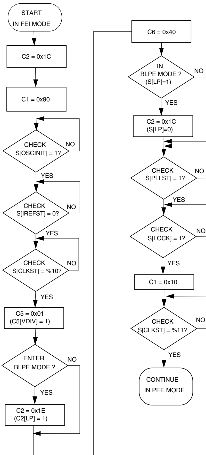
Figure 24-13. Flowchart of FEI to PEE Mode Transition using an 4 MHz crystal K50 Sub-Family Reference Manual, Rev. 6, Nov 2011
