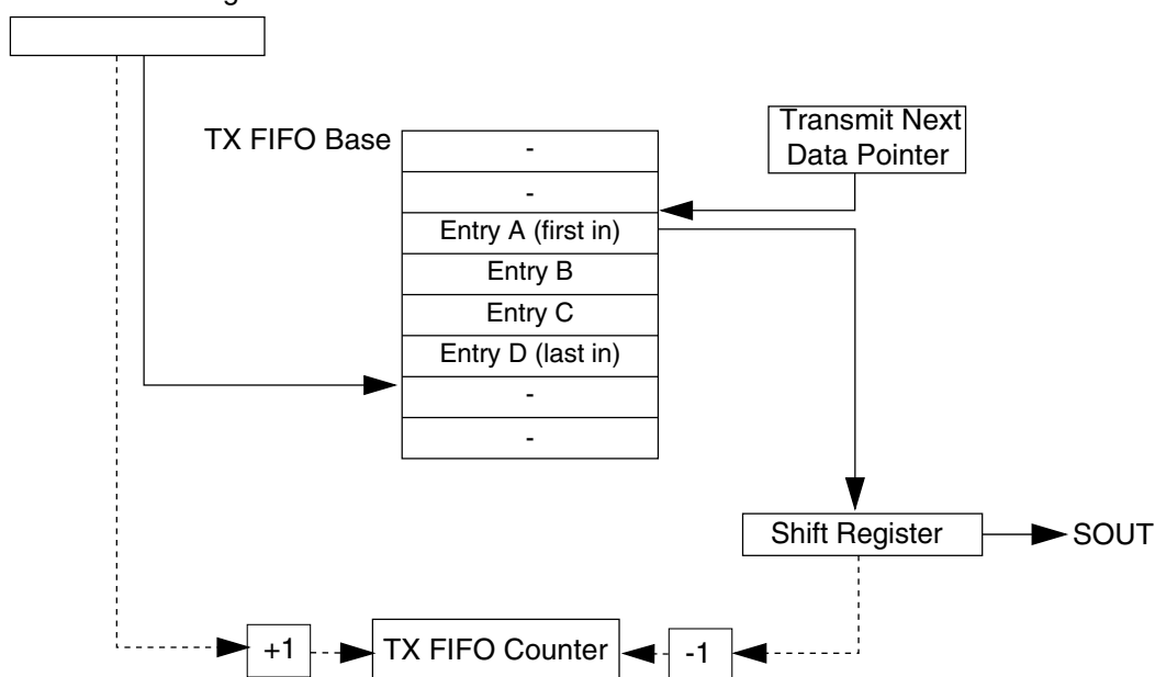
Figure 47-100. TX FIFO Pointers and Counter
