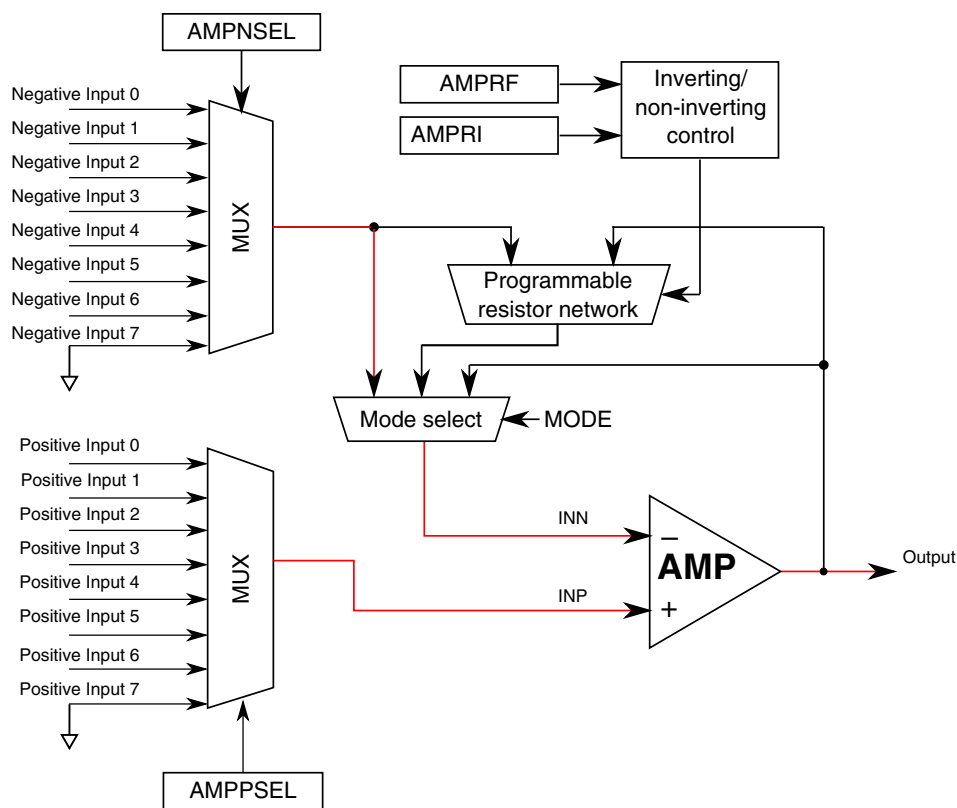
Figure 35-11. Operational Amplifier Block Diagram in General Purpose Mode
