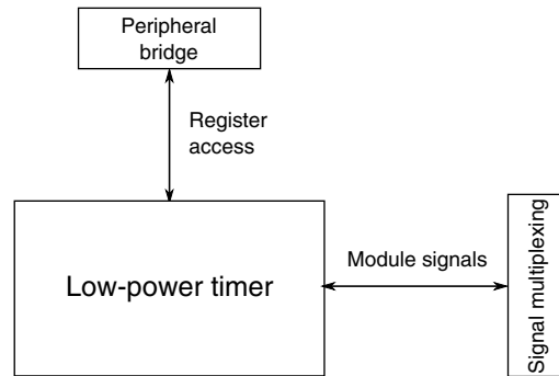
Figure 3-47. LPT configuration
