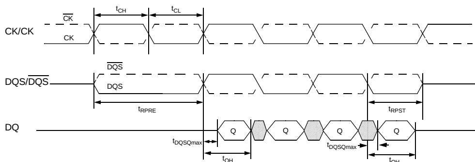
&lt;Data output (read) timing&gt;
