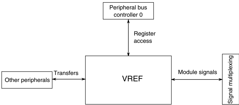
Figure 3-40. VREF configuration
