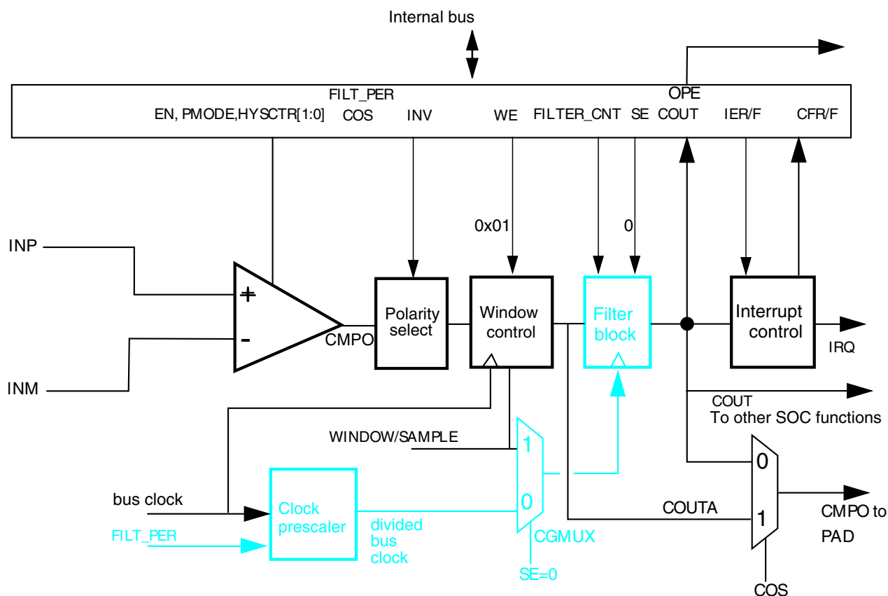
Figure 34-33. Windowed mode
