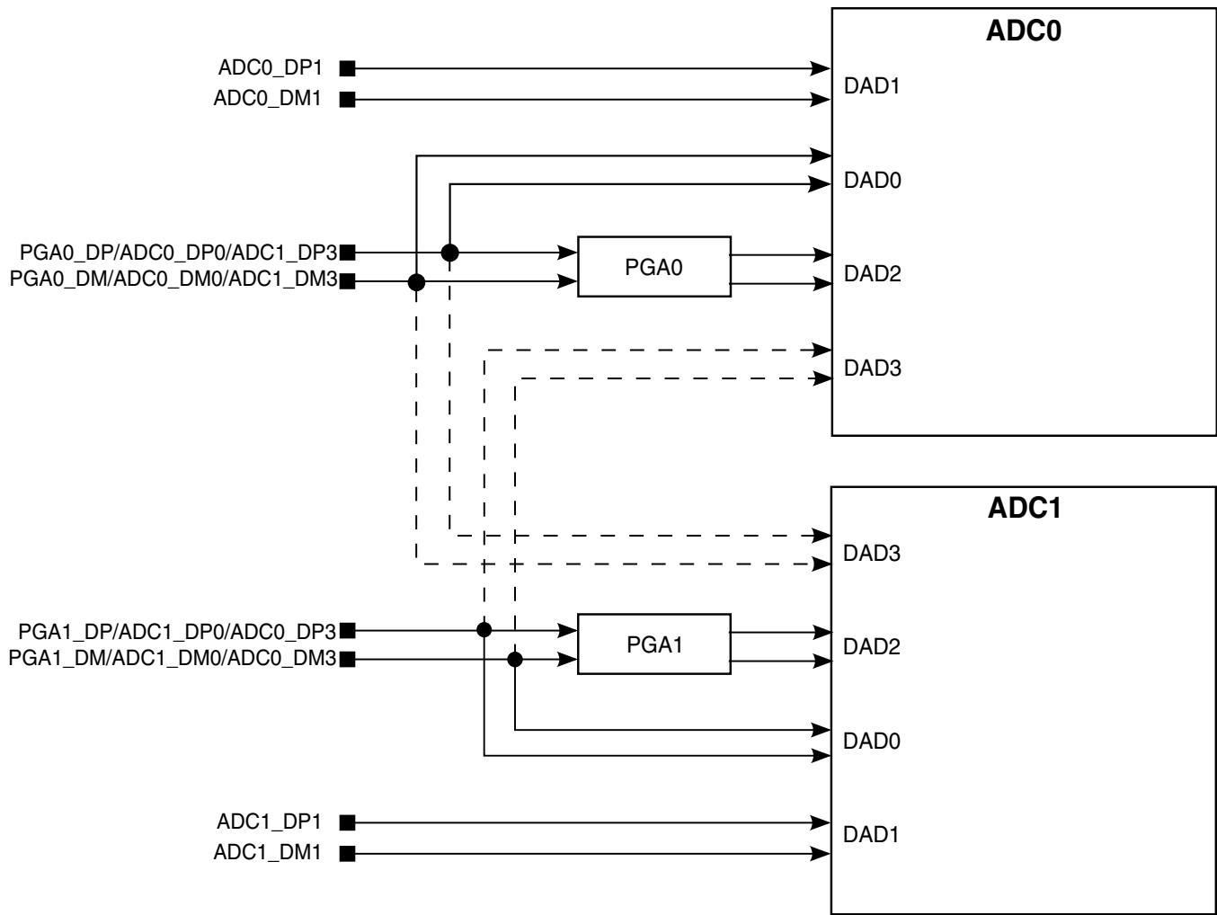
Figure 3-37. PGA Integration
