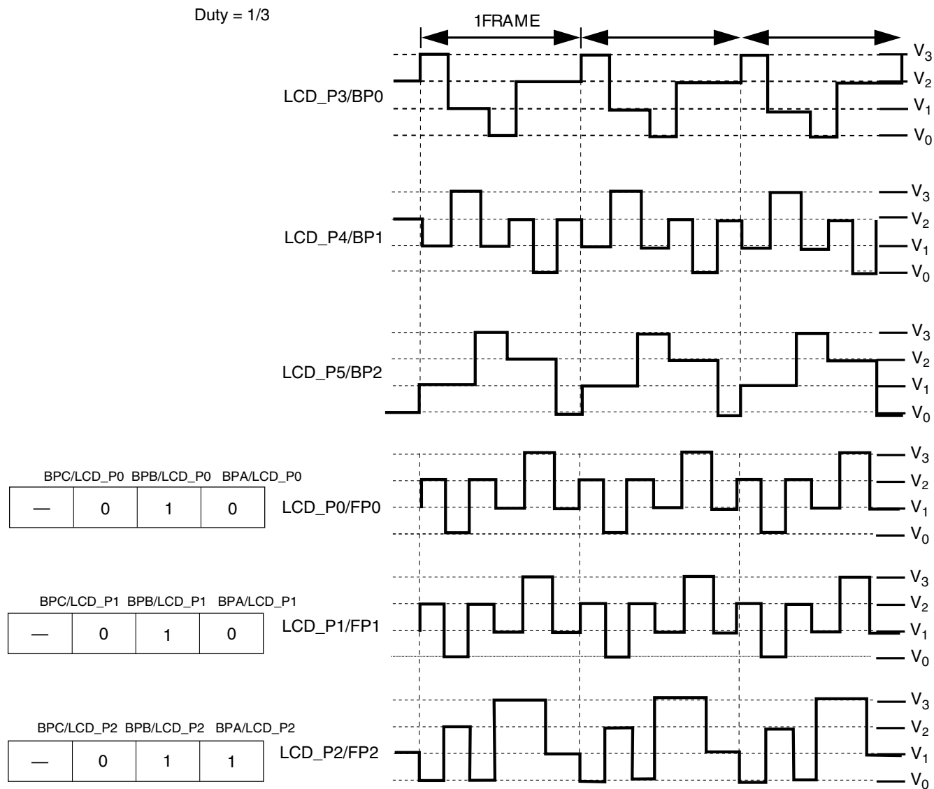
Figure 54-40. LCD waveforms
