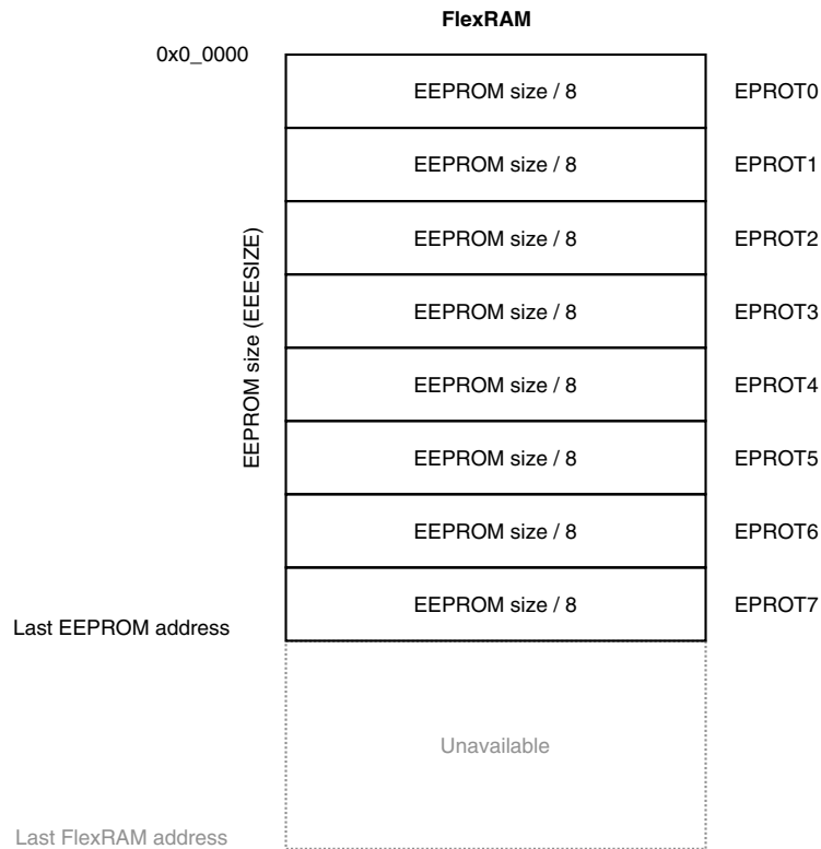
Figure 29-30. EEPROM protection
