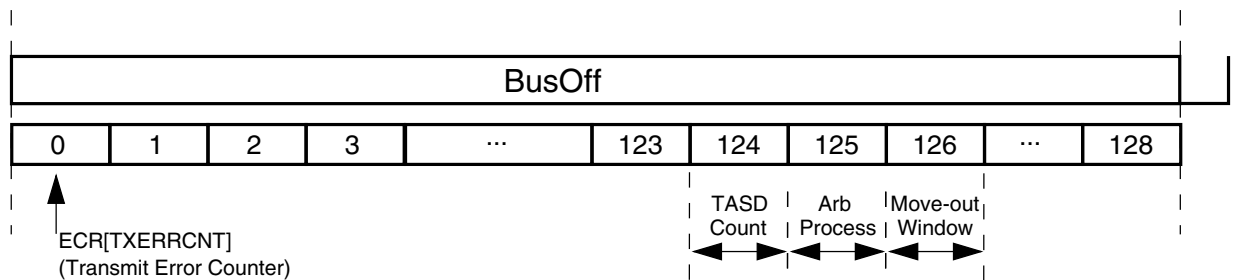
Figure 46-102. Arbitration at the end of bus off and move-out time windows
