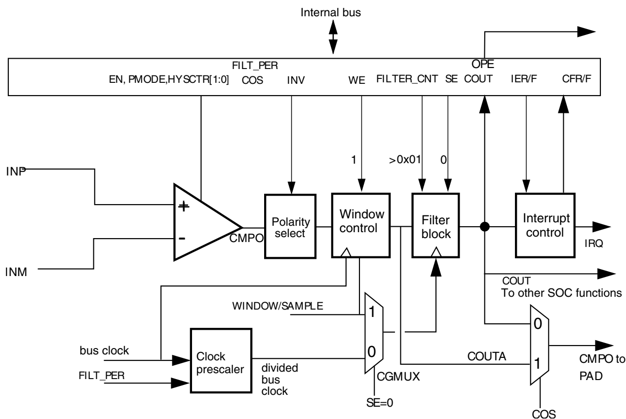
Figure 34-35. Windowed/Filtered mode
