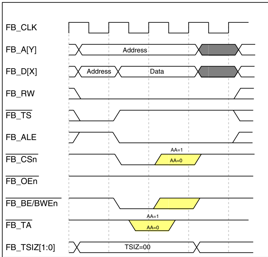
Figure 30-34. Longword-Write Transfer
