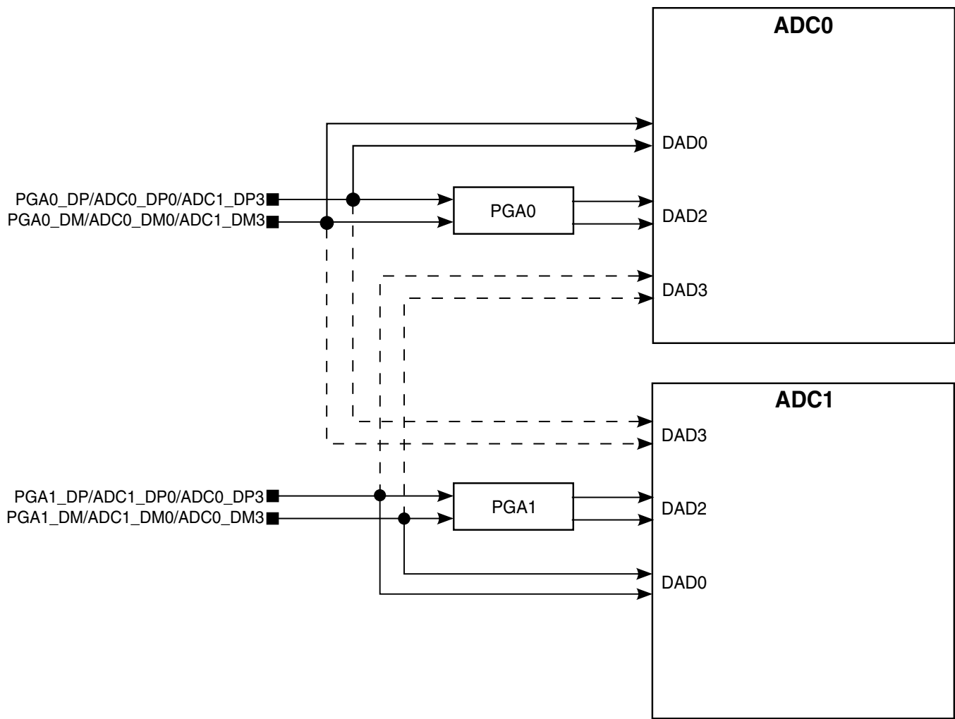
Figure 3-34. PGA Integration
