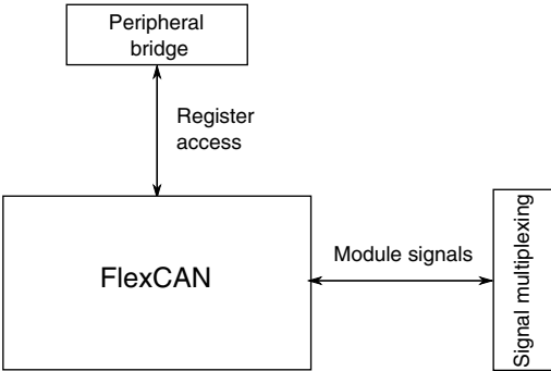
Figure 3-54. CAN configuration
