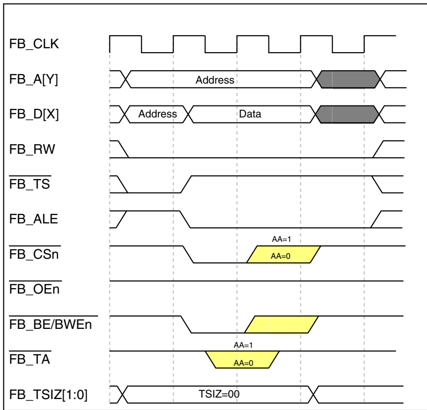
Figure 29-34. Longword-Write Transfer
