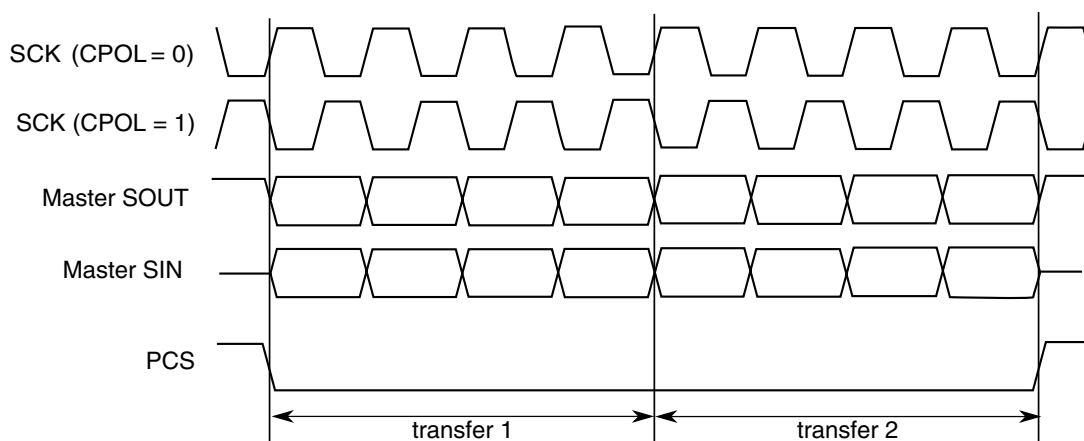
Figure 43-54. Continuous SCK timing diagram (CONT=1)
