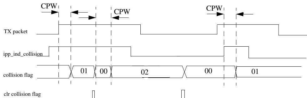
Figure 45-197. Collision pulse detection
