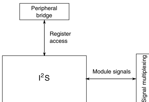
Figure 3-51. I²S configuration
