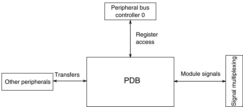
Figure 3-32. PDB configuration
