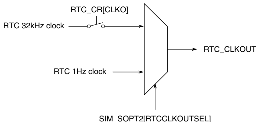
Figure 3-40. RTC_CLKOUT generation
