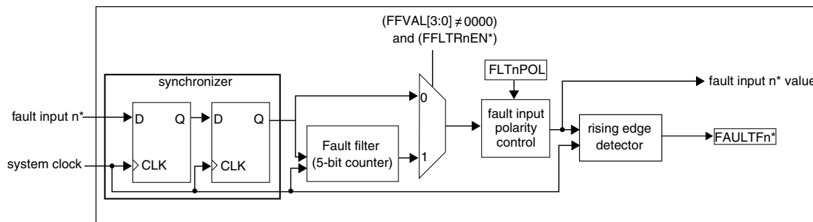
Figure 35-192. Fault input n control block diagram
