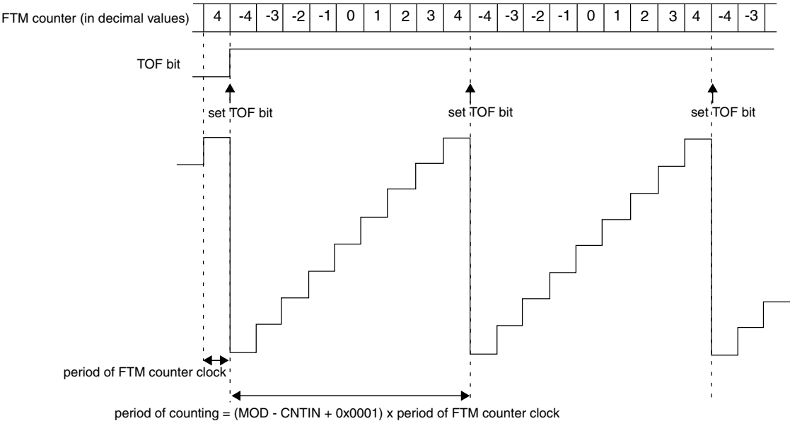
Figure 35-127. Example of FTM up and signed counting
