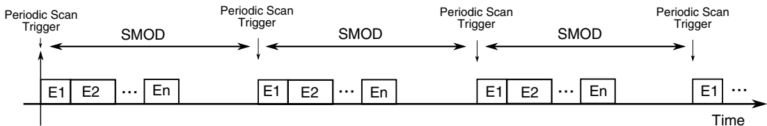
Figure 47-40. Periodical Scan Time Chart
