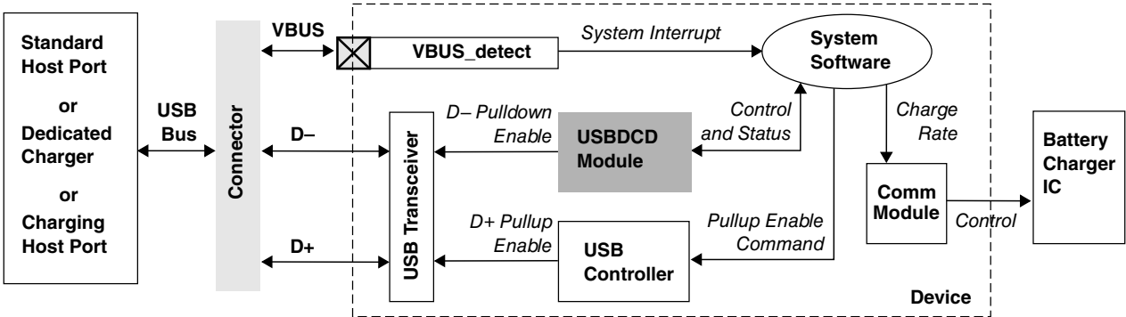
Figure 40-8. USB battery charging subsystem
