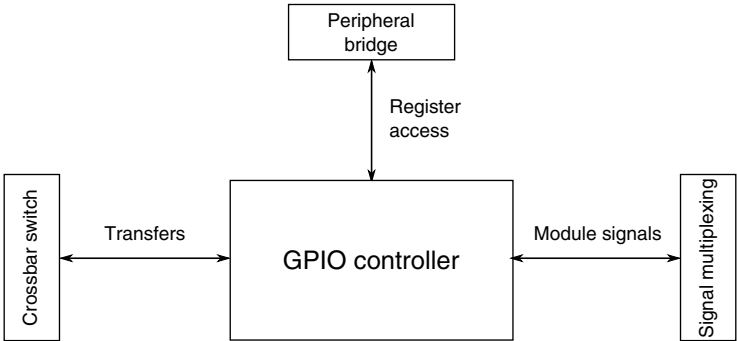
Figure 3-51. GPIO configuration
