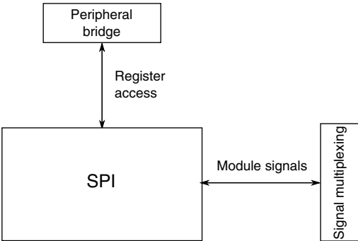
Figure 3-47. SPI configuration
