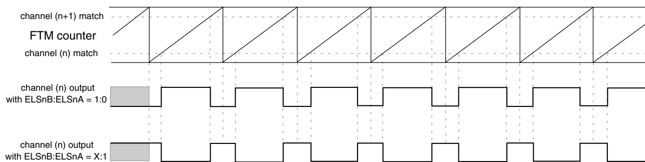
Figure 34-146. Combine mode
