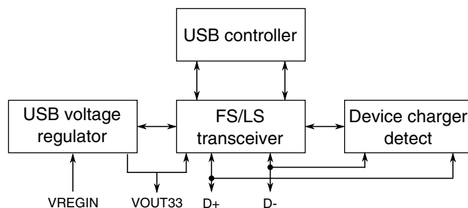
Figure 3-40. USB Subsystem Overview
