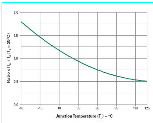
Figure 5: Normalized DC Holding Current vs. Junction Temperature
