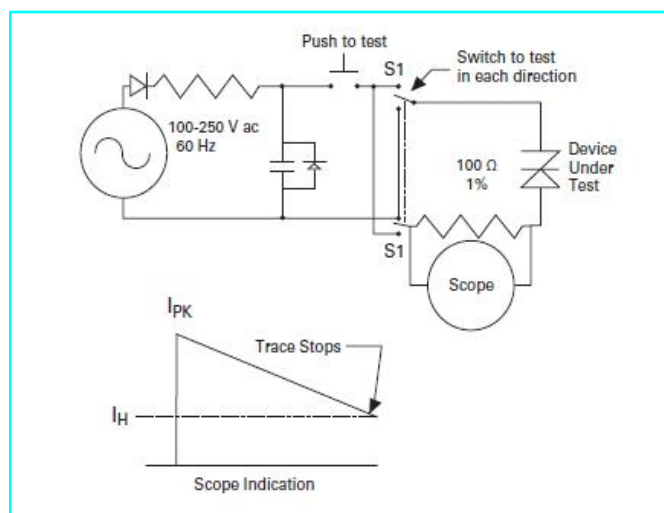
Figure 6: Dynamic Holding Current Test Circuit for SIDACs
