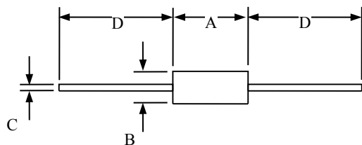
DO-15
