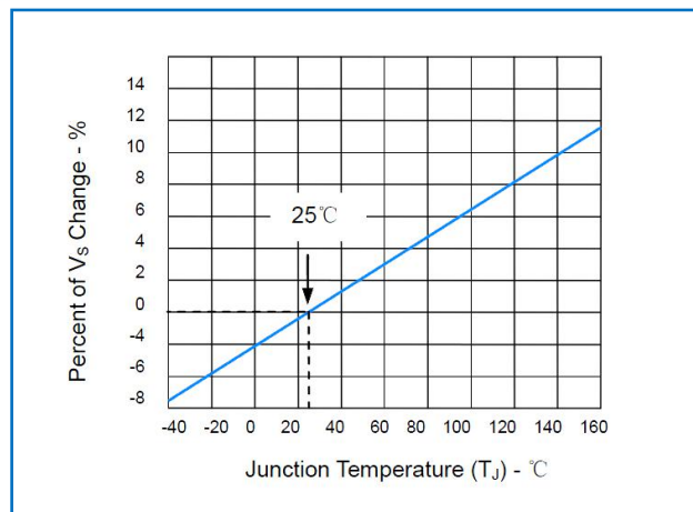
Figure 1- Normalized V s change vs. junction temperature
