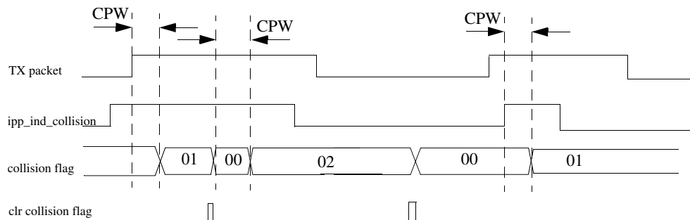
Figure 45-245. Collision pulse detection
