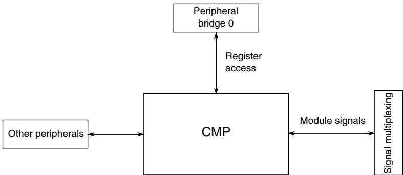
Figure 3-35. CMP configuration
