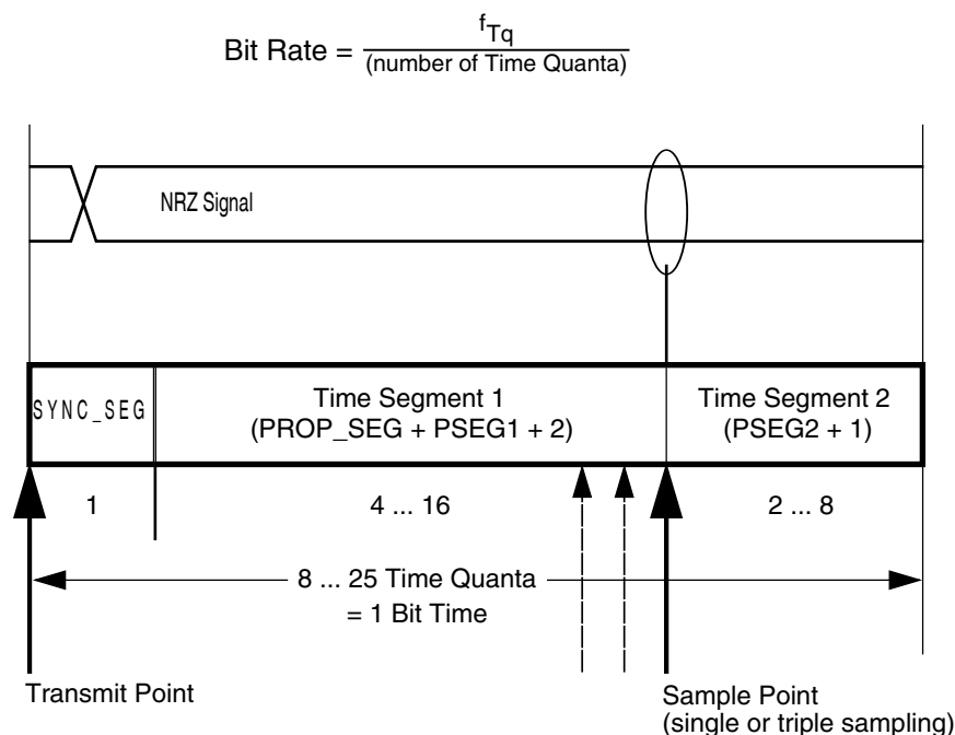
Figure 42-67. Segments within the bit time
