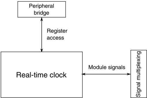
Figure 3-45. RTC configuration
