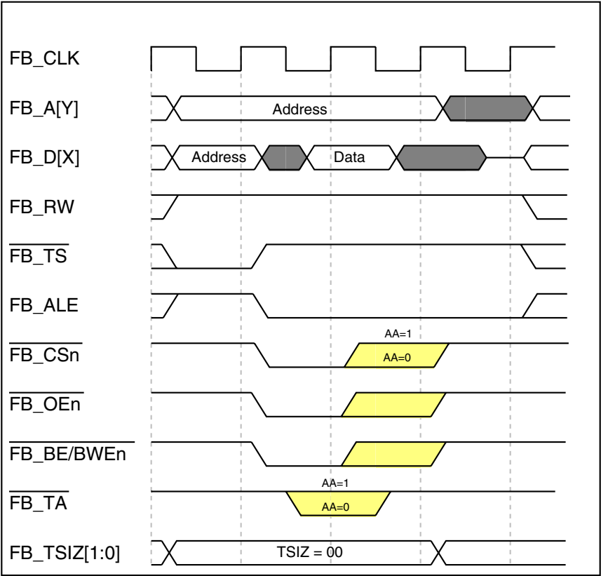
Figure 29-33. Longword-Read Transfer
