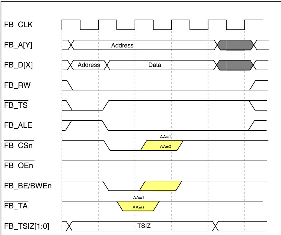
Figure 29-42. Write Cycle with Two-Clock Address Hold (No Wait States)
