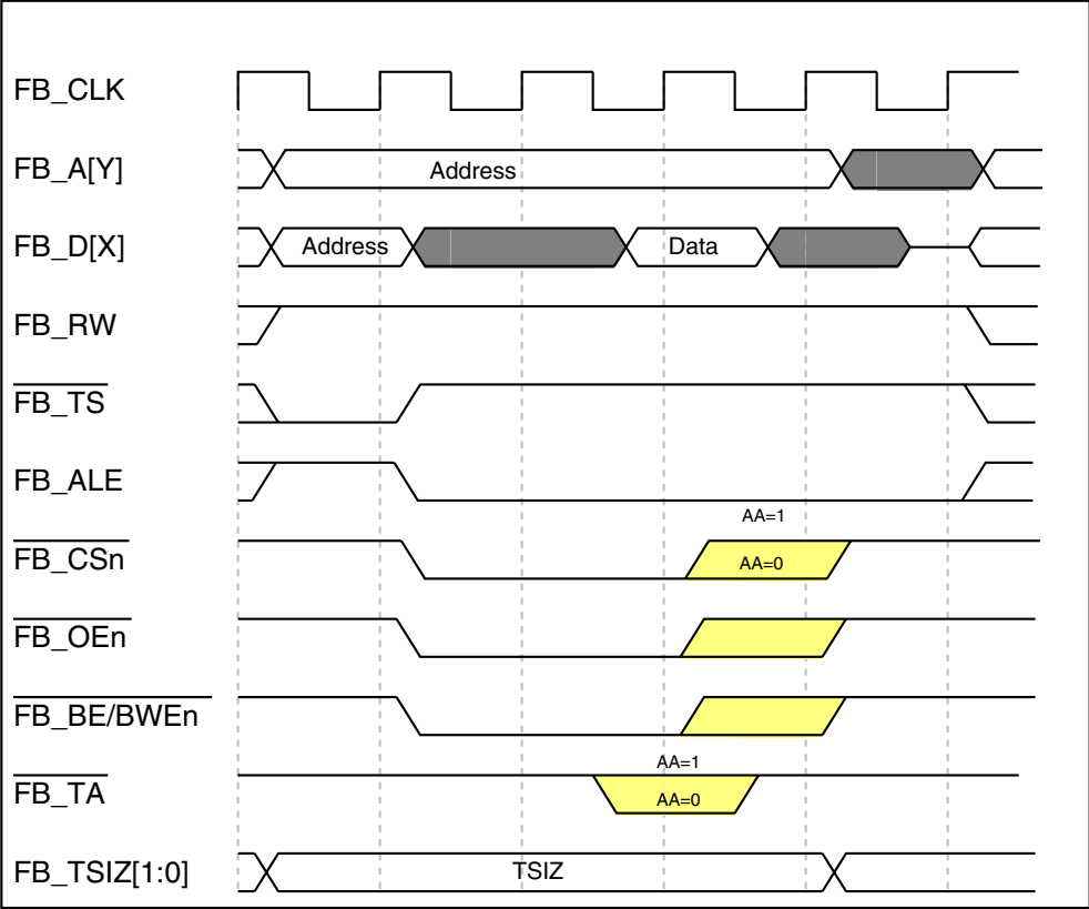
Figure 29-37. Read-Bus Cycle (One Wait State)
