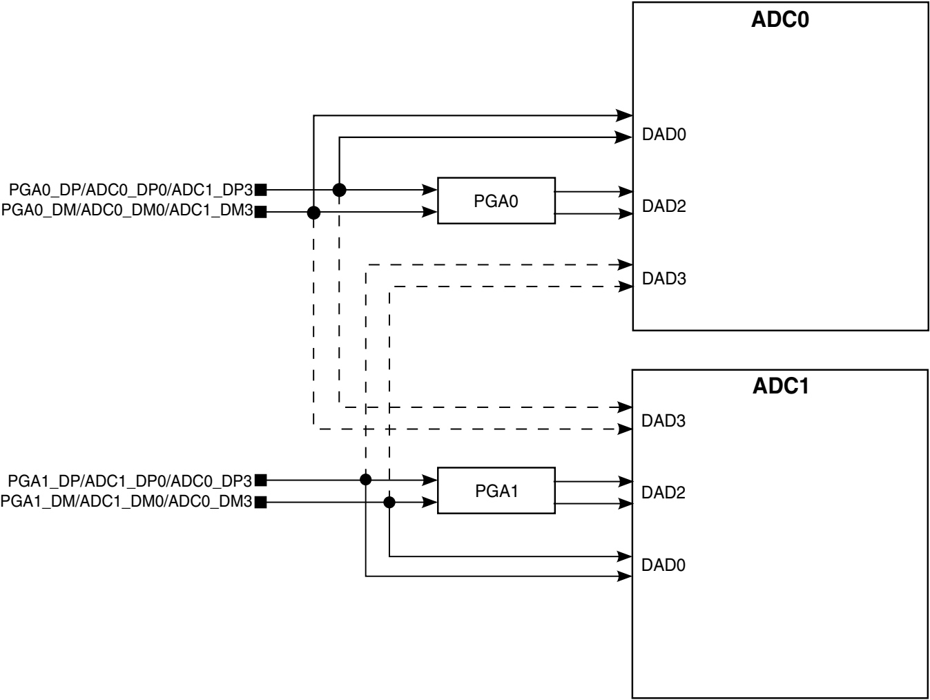
Figure 3-34. PGA Integration
