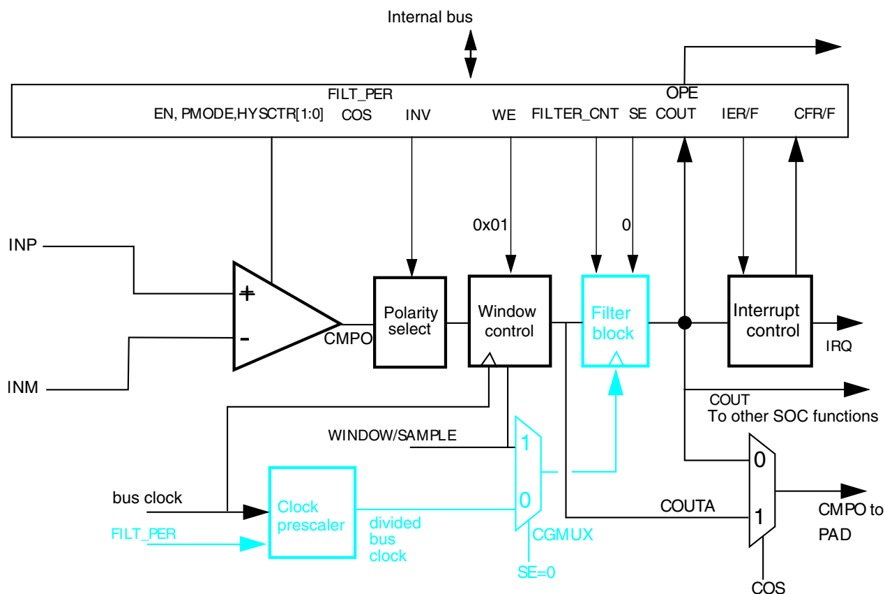
Figure 33-33. Windowed mode
