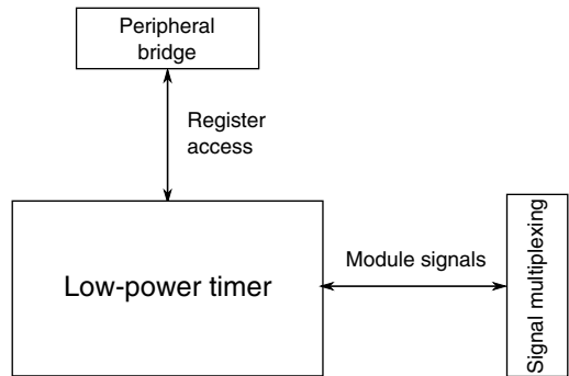
Figure 3-43. LPT configuration
