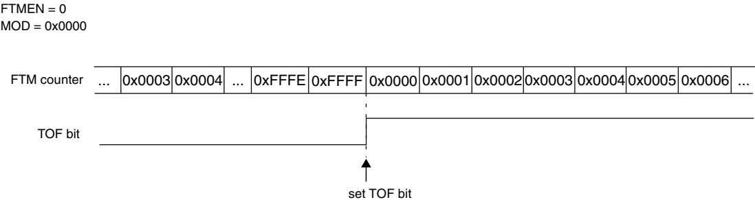
Figure 37-172. Example when the FTM counter is free running
