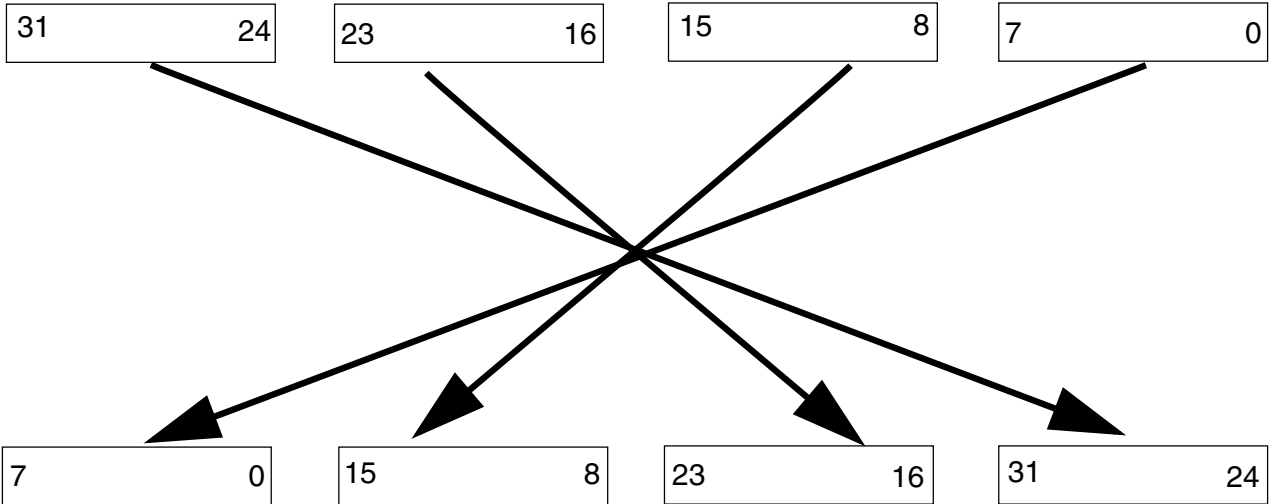
Figure 31-7. Transpose type 11
