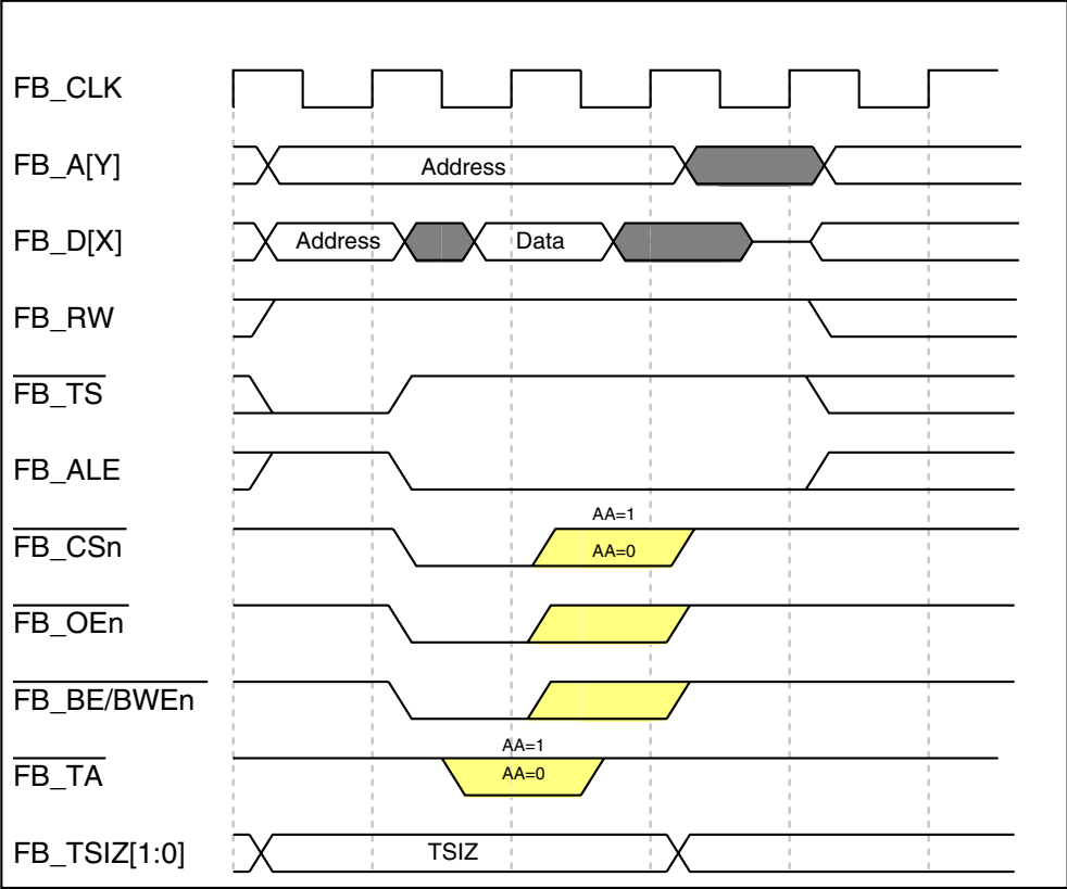
Figure 29-35. Basic Read-Bus Cycle (No Wait States)
