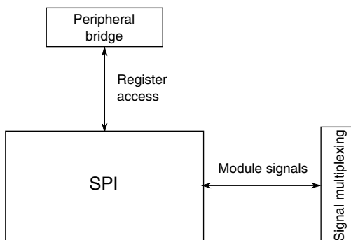
Figure 3-48. SPI configuration
