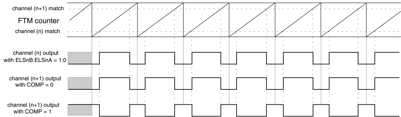
Figure 37-203. Channel (n+1) output in Complementary mode with (ELSnB:ELSnA = 1:0)
