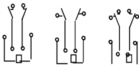
wiring diagram(bottom views)
