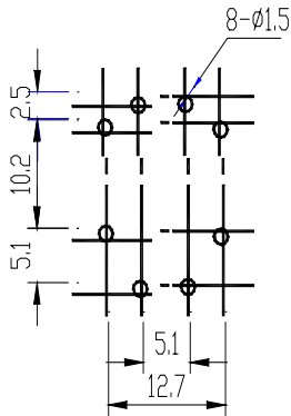
Mounting (Bottom views)
