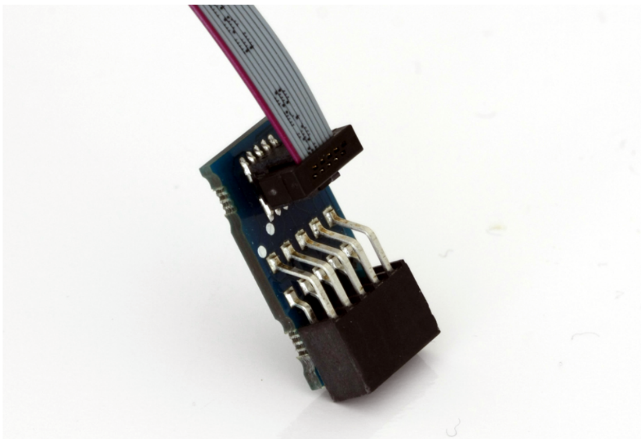
Figure 2-5. JTAGICE3 Probe Adapter Connection
